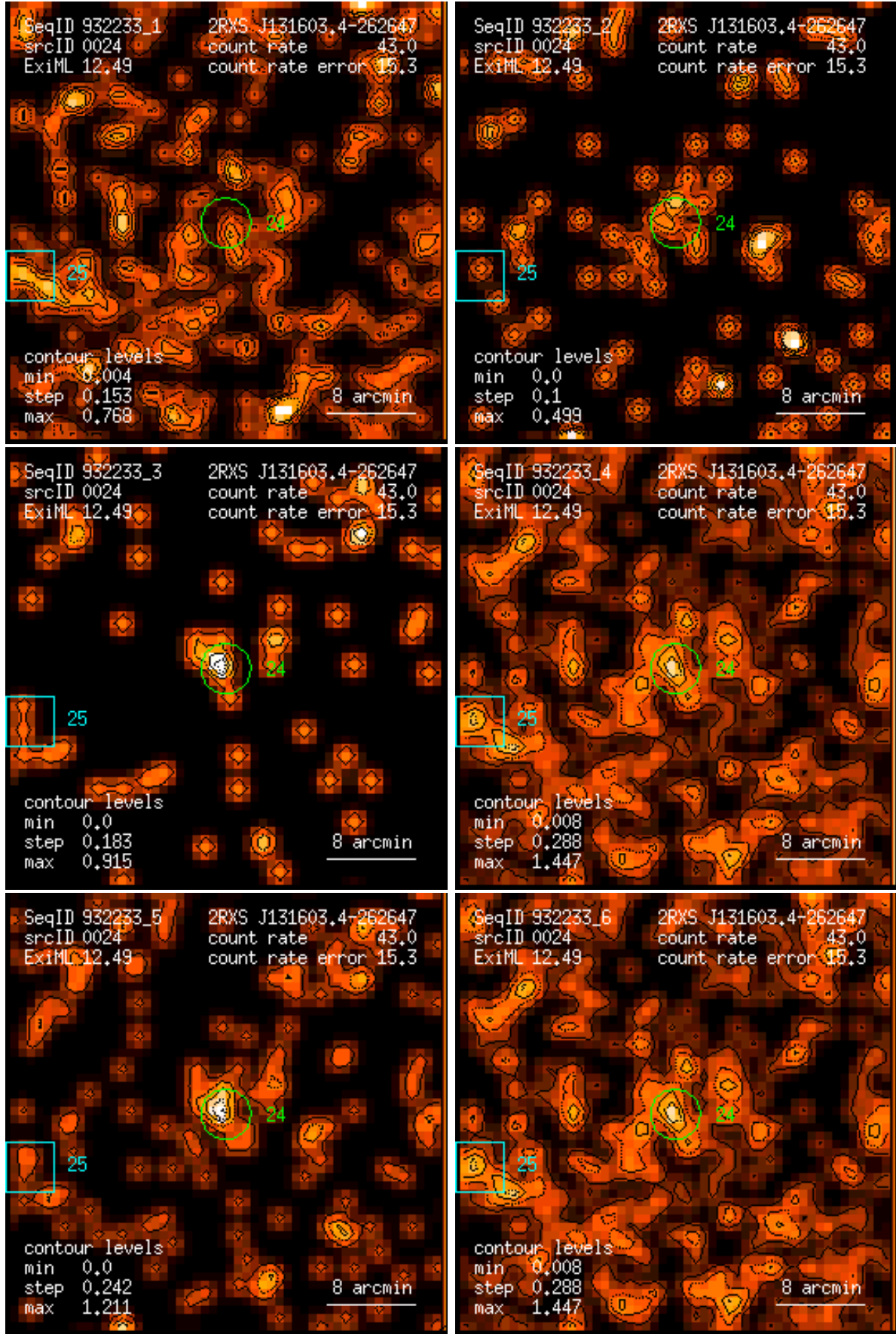
Figure 24: RASS 932233: detection 0024: band rate images, Gaussian filter: (1) PSPC channels 11 – 41, (2) 52 – 90, (3) 91 – 201, (4) 11 – 235, (5) 52 – 201, (6) 11 – 201. Broad band rates in counts/ks. Band rate contour levels in counts/ks/arcmin 2 .
