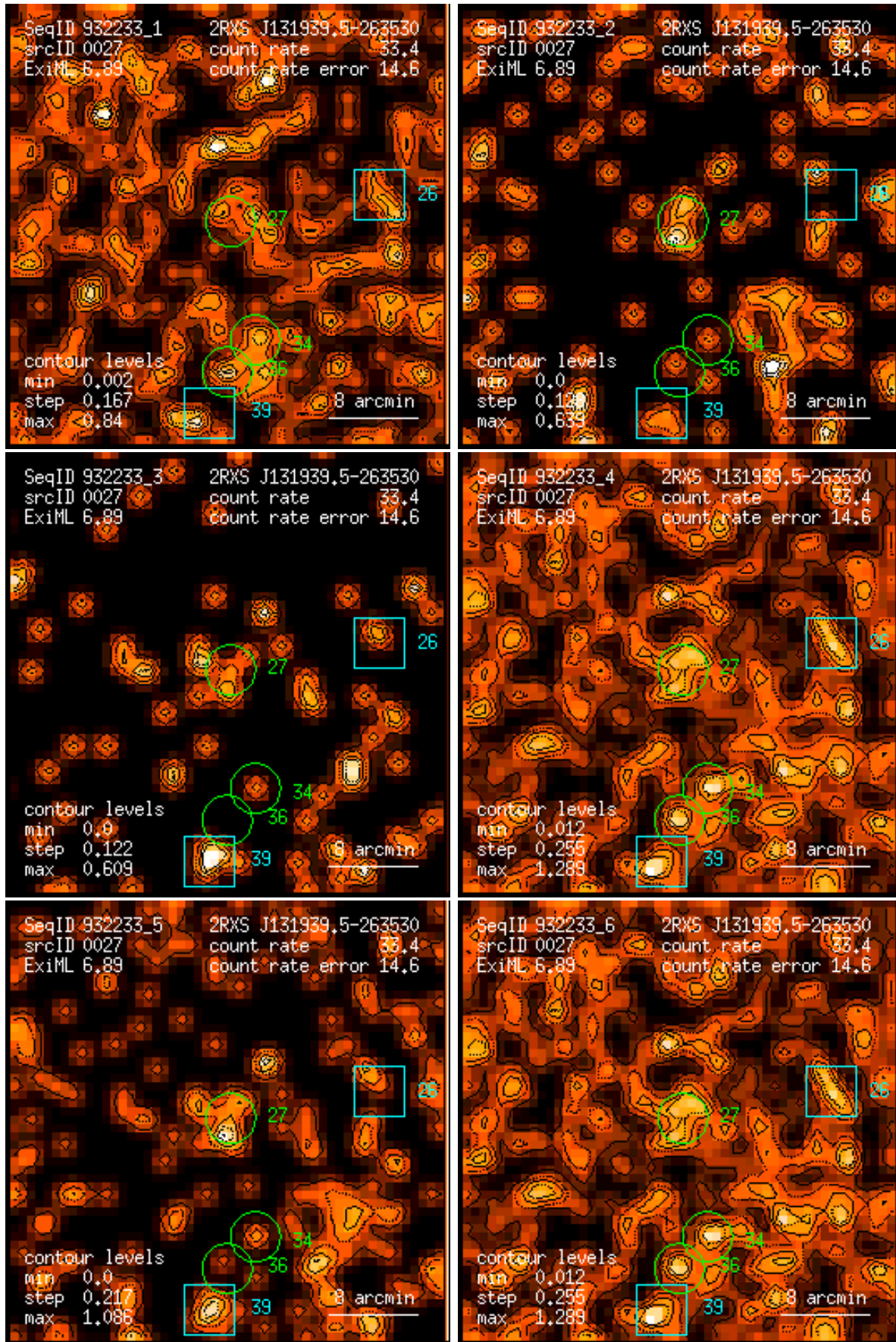
Figure 27: RASS 932233: detection 0027: band rate images, Gaussian filter: (1) PSPC channels 11 – 41, (2) 52 – 90, (3) 91 – 201, (4) 11 – 235, (5) 52 – 201, (6) 11 – 201. Broad band rates in counts/ks. Band rate contour levels in counts/ks/arcmin 2 .
