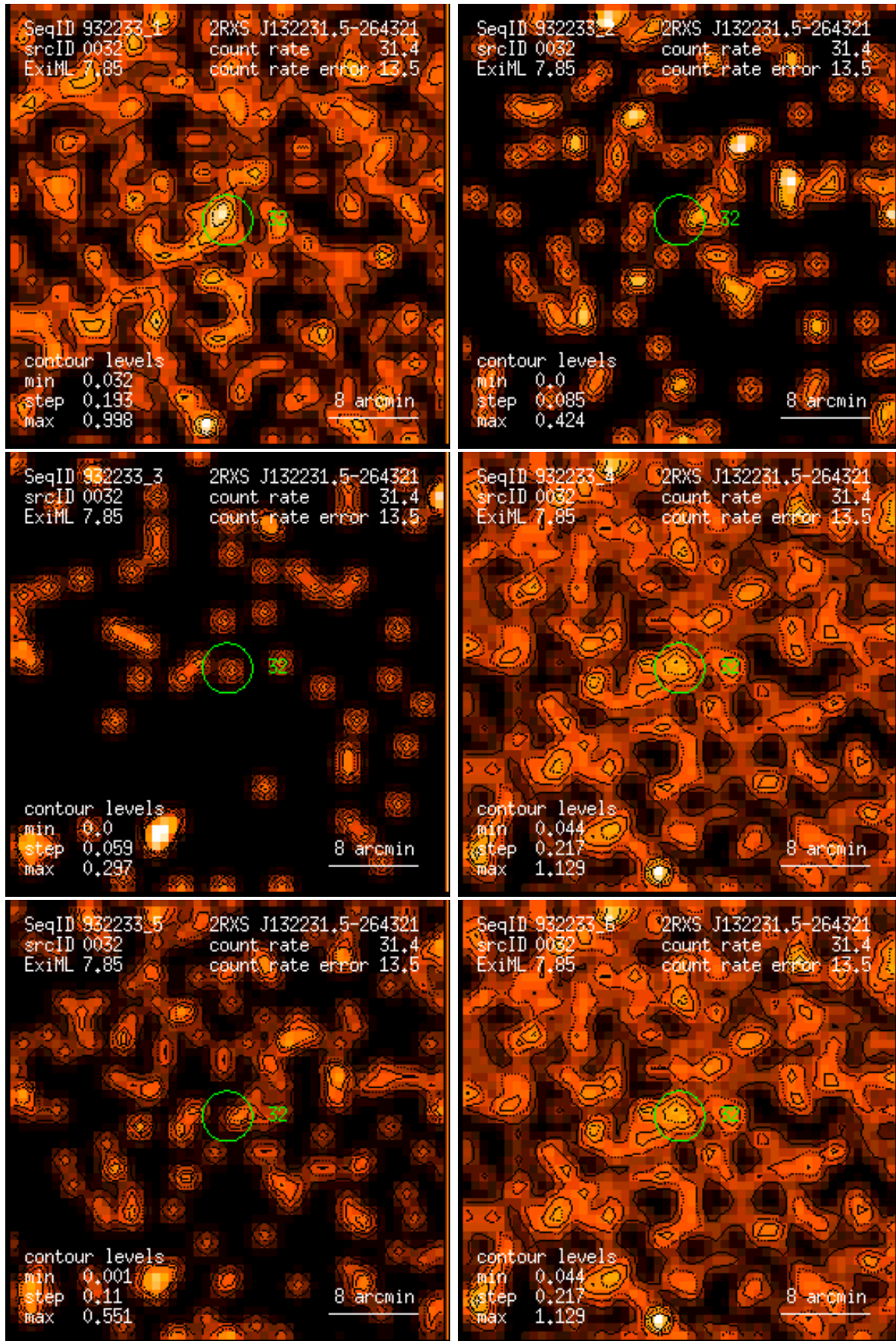
Figure 32: RASS 932233: detection 0032: band rate images, Gaussian filter: (1) PSPC channels 11 – 41, (2) 52 – 90, (3) 91 – 201, (4) 11 – 235, (5) 52 – 201, (6) 11 – 201. Broad band rates in counts/ks. Band rate contour levels in counts/ks/arcmin 2 .
