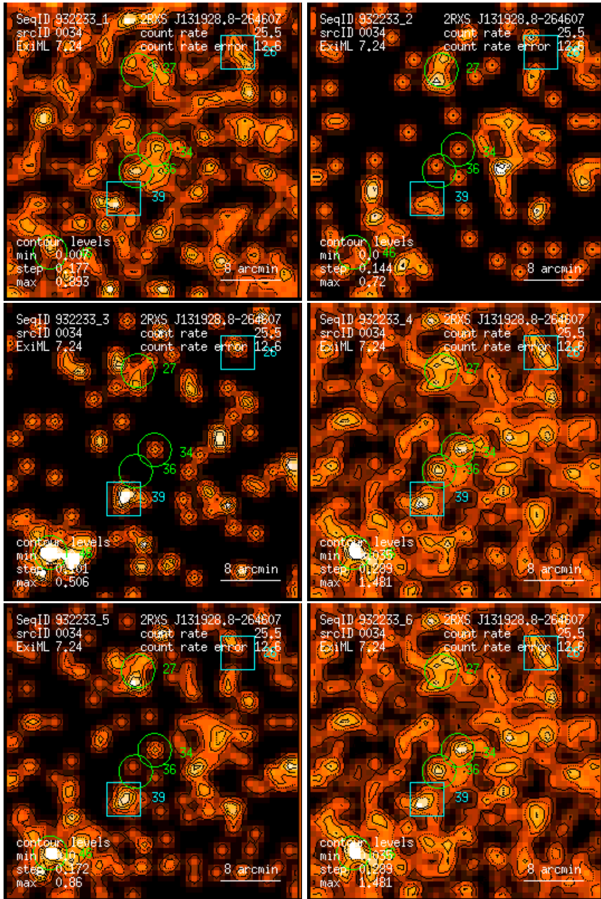
Figure 34: RASS 932233: detection 0034: band rate images, Gaussian filter: (1) PSPC channels 11 – 41, (2) 52 – 90, (3) 91 – 201, (4) 11 – 235, (5) 52 – 201, (6) 11 – 201. Broad band rates in counts/ks. Band rate contour levels in counts/ks/arcmin 2 .
