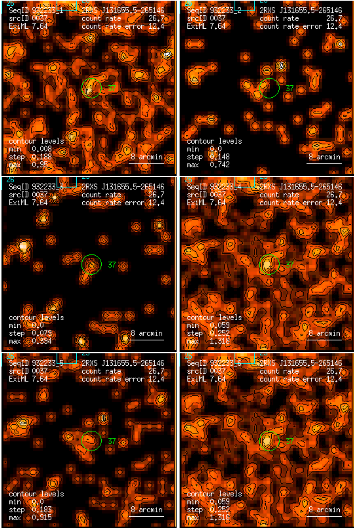
Figure 37: RASS 932233: detection 0037: band rate images, Gaussian filter: (1) PSPC channels 11 – 41, (2) 52 – 90, (3) 91 – 201, (4) 11 – 235, (5) 52 – 201, (6) 11 – 201. Broad band rates in counts/ks. Band rate contour levels in counts/ks/arcmin 2 .
