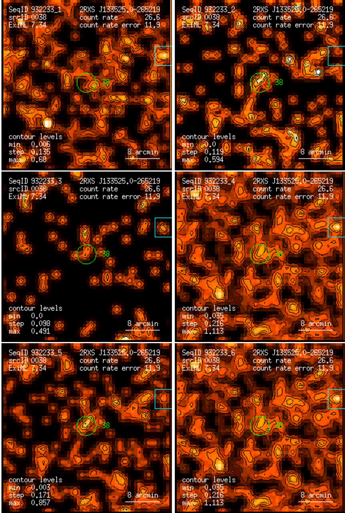
Figure 38: RASS 932233: detection 0038: band rate images, Gaussian filter: (1) PSPC channels 11 – 41, (2) 52 – 90, (3) 91 – 201, (4) 11 – 235, (5) 52 – 201, (6) 11 – 201. Broad band rates in counts/ks. Band rate contour levels in counts/ks/arcmin 2 .
