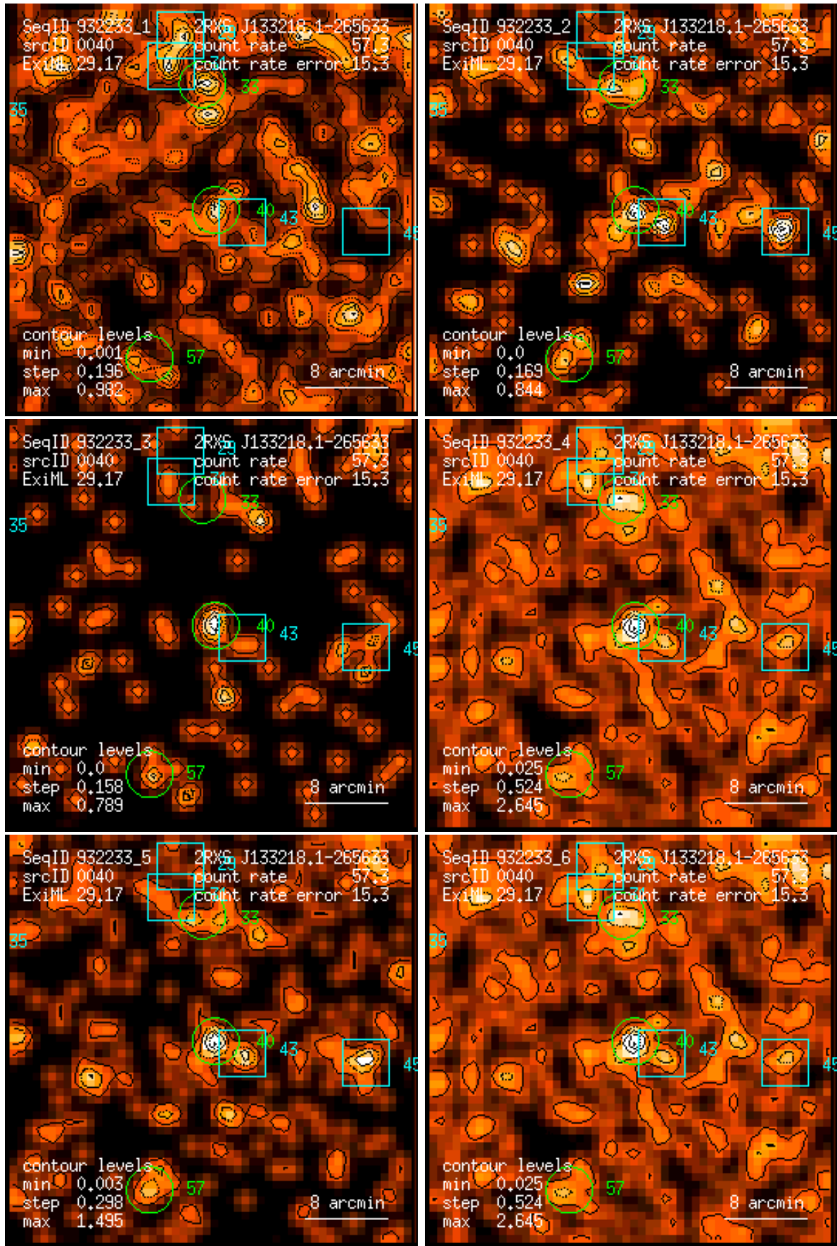
Figure 40: RASS 932233: detection 0040: band rate images, Gaussian filter: (1) PSPC channels 11 – 41, (2) 52 – 90, (3) 91 – 201, (4) 11 – 235, (5) 52 – 201, (6) 11 – 201. Broad band rates in counts/ks. Band rate contour levels in counts/ks/arcmin 2 .
