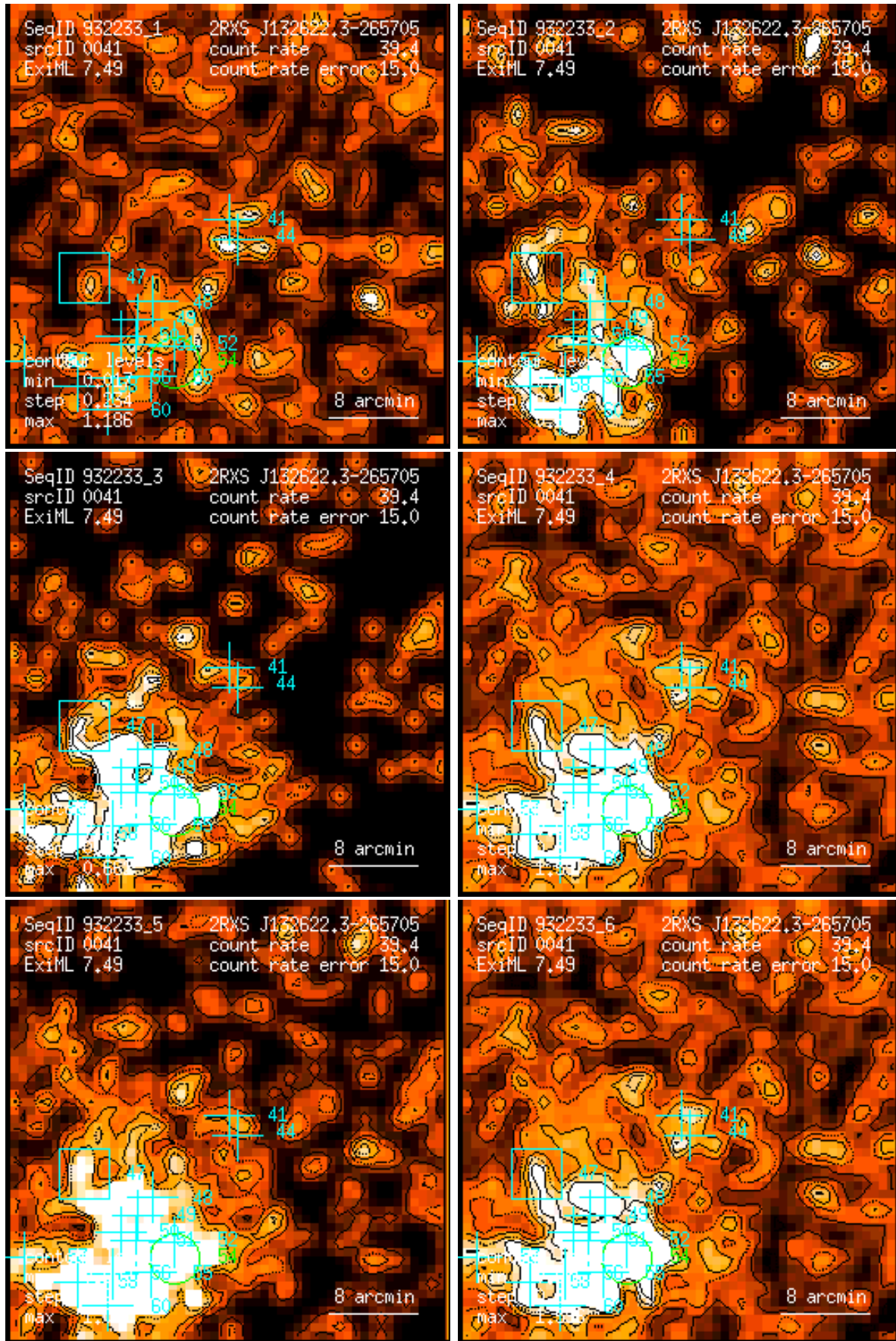
Figure 41: RASS 932233: detection 0041: band rate images, Gaussian filter: (1) PSPC channels 11 – 41, (2) 52 – 90, (3) 91 – 201, (4) 11 – 235, (5) 52 – 201, (6) 11 – 201. Broad band rates in counts/ks. Band rate contour levels in counts/ks/arcmin 2 .
