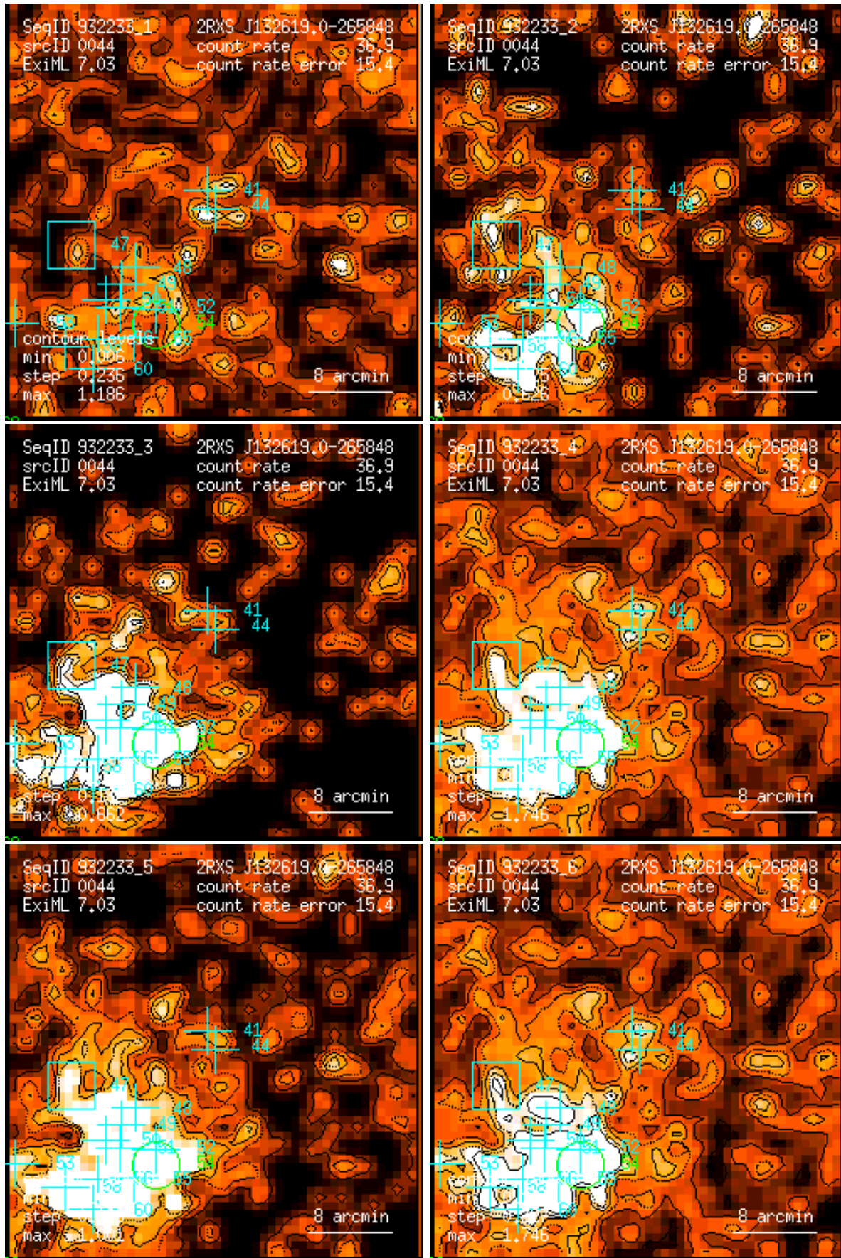
Figure 44: RASS 932233: detection 0044: band rate images, Gaussian filter: (1) PSPC channels 11 – 41, (2) 52 – 90, (3) 91 – 201, (4) 11 – 235, (5) 52 – 201, (6) 11 – 201. Broad band rates in counts/ks. Band rate contour levels in counts/ks/arcmin 2 .
