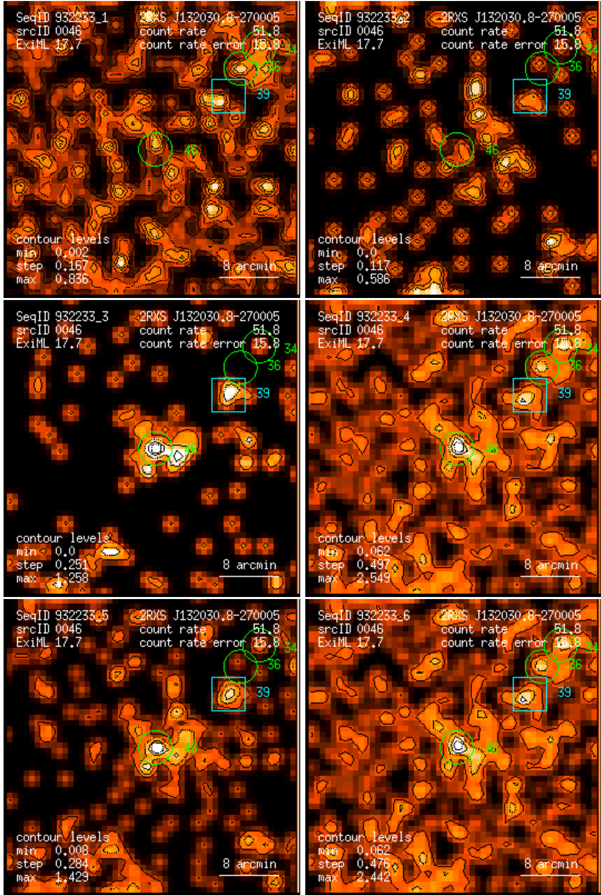
Figure 46: RASS 932233: detection 0046: band rate images, Gaussian filter: (1) PSPC channels 11 – 41, (2) 52 – 90, (3) 91 – 201, (4) 11 – 235, (5) 52 – 201, (6) 11 – 201. Broad band rates in counts/ks. Band rate contour levels in counts/ks/arcmin 2 .
