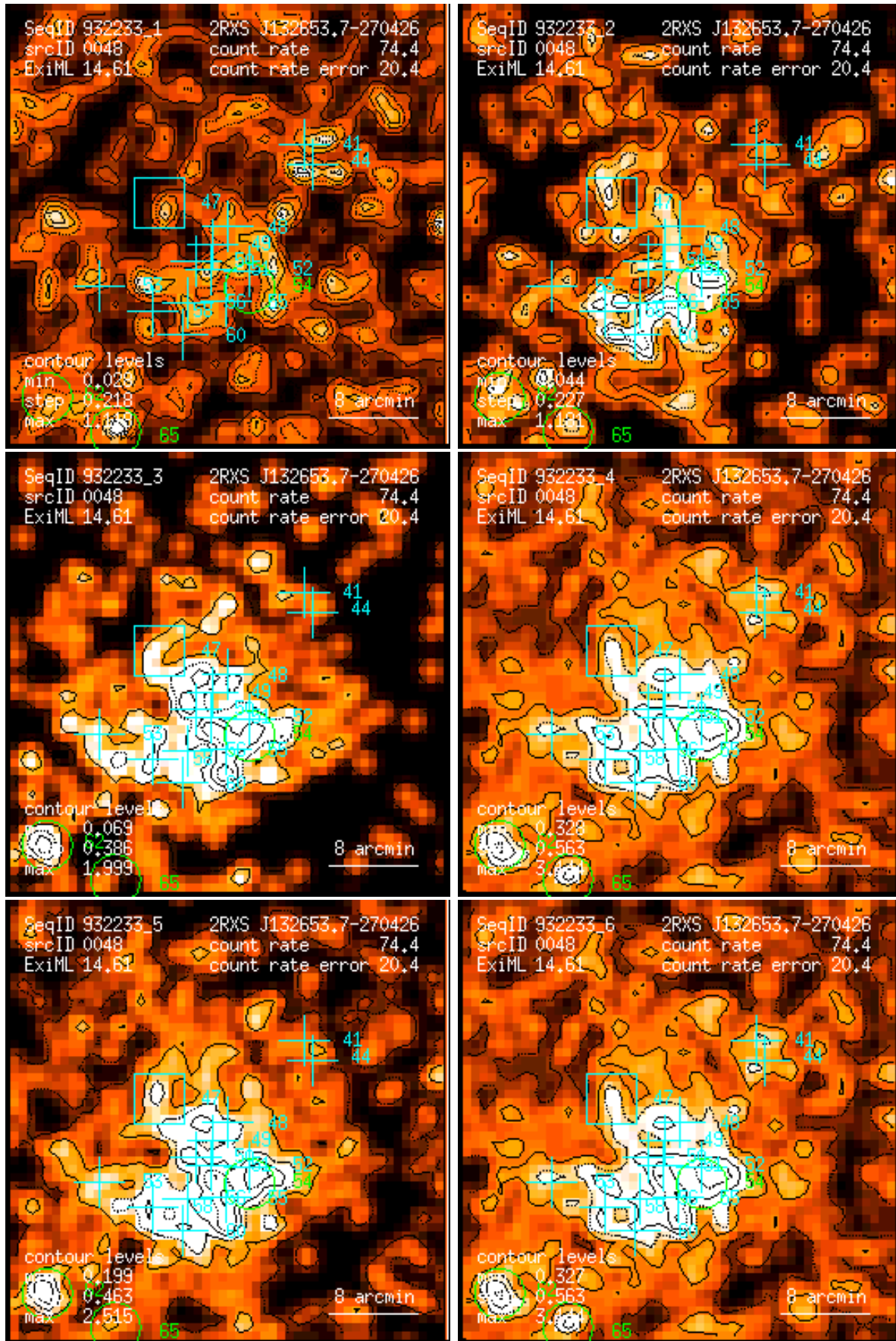
Figure 48: RASS 932233: detection 0048: band rate images, Gaussian filter: (1) PSPC channels 11 – 41, (2) 52 – 90, (3) 91 – 201, (4) 11 – 235, (5) 52 – 201, (6) 11 – 201. Broad band rates in counts/ks. Band rate contour levels in counts/ks/arcmin 2 .
