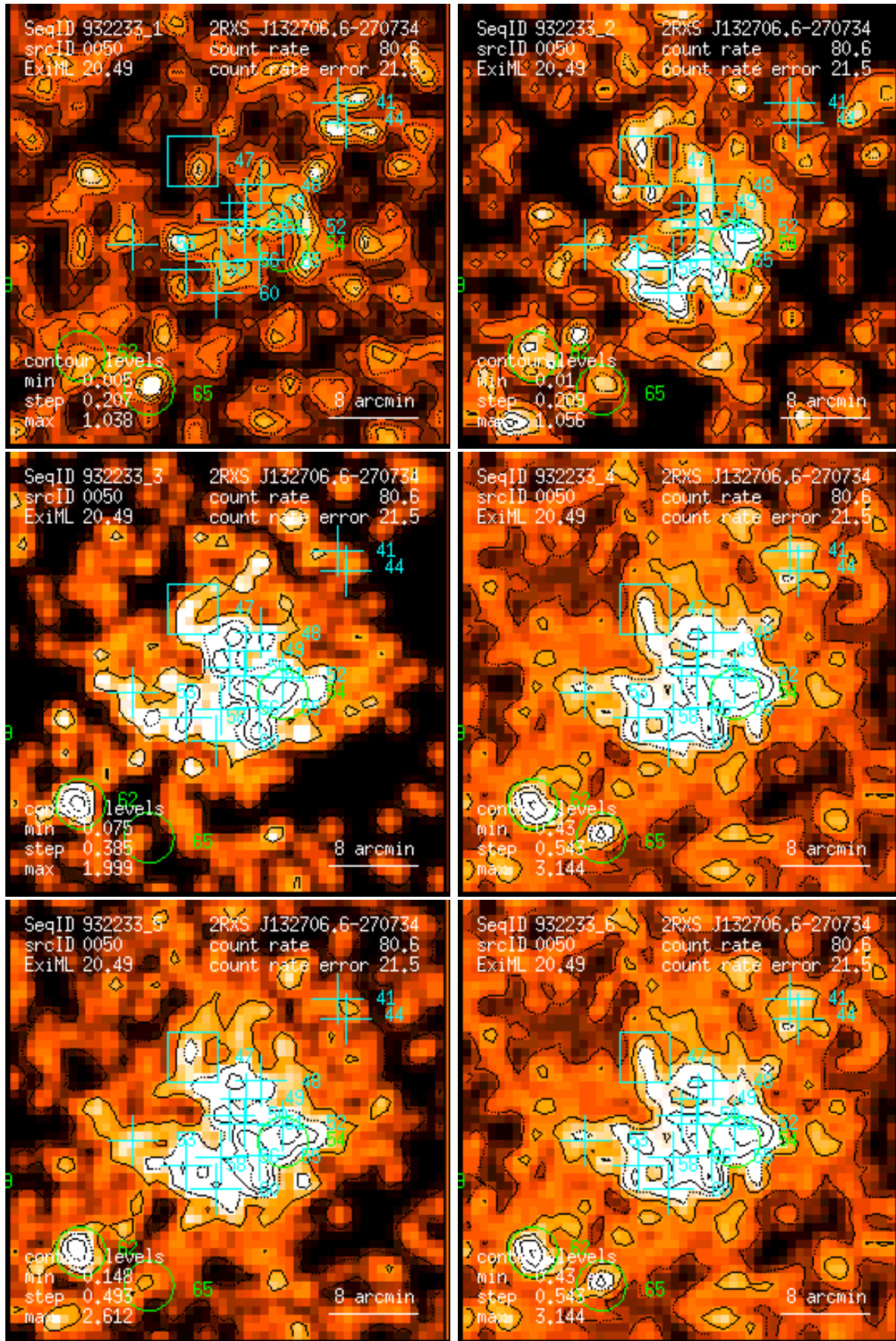
Figure 50: RASS 932233: detection 0050: band rate images, Gaussian filter: (1) PSPC channels 11 – 41, (2) 52 – 90, (3) 91 – 201, (4) 11 – 235, (5) 52 – 201, (6) 11 – 201. Broad band rates in counts/ks. Band rate contour levels in counts/ks/arcmin 2 .
