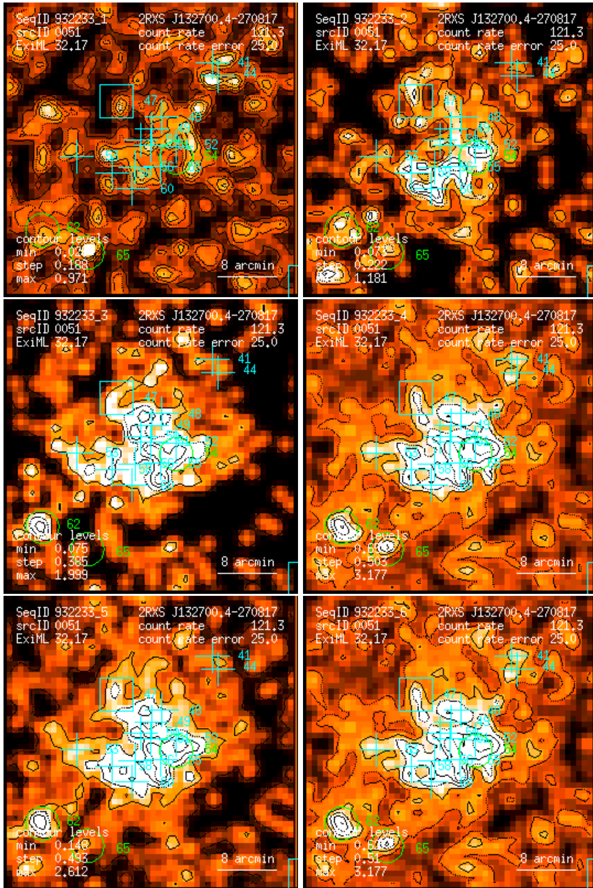
Figure 51: RASS 932233: detection 0051: band rate images, Gaussian filter: (1) PSPC channels 11 – 41, (2) 52 – 90, (3) 91 – 201, (4) 11 – 235, (5) 52 – 201, (6) 11 – 201. Broad band rates in counts/ks. Band rate contour levels in counts/ks/arcmin 2 .
