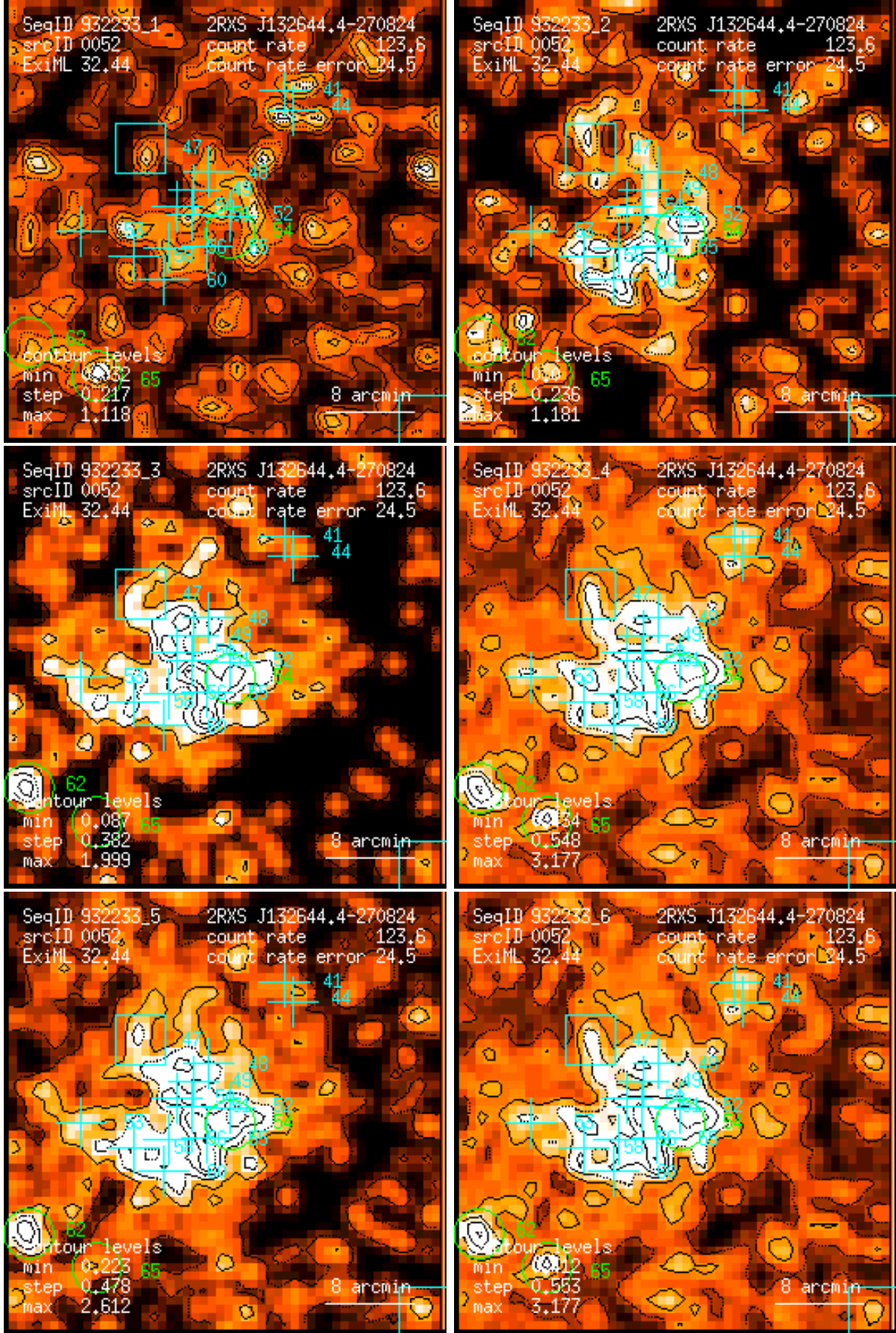
Figure 52: RASS 932233: detection 0052: band rate images, Gaussian filter: (1) PSPC channels 11 – 41, (2) 52 – 90, (3) 91 – 201, (4) 11 – 235, (5) 52 – 201, (6) 11 – 201. Broad band rates in counts/ks. Band rate contour levels in counts/ks/arcmin 2 .
