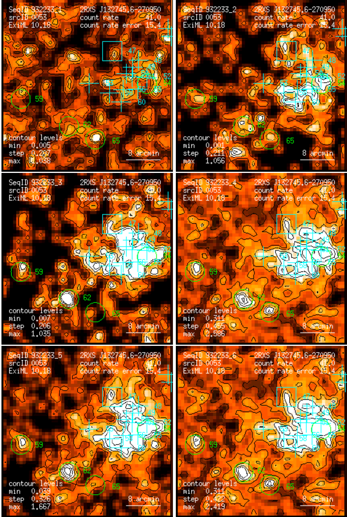
Figure 53: RASS 932233: detection 0053: band rate images, Gaussian filter: (1) PSPC channels 11 – 41, (2) 52 – 90, (3) 91 – 201, (4) 11 – 235, (5) 52 – 201, (6) 11 – 201. Broad band rates in counts/ks. Band rate contour levels in counts/ks/arcmin 2 .
