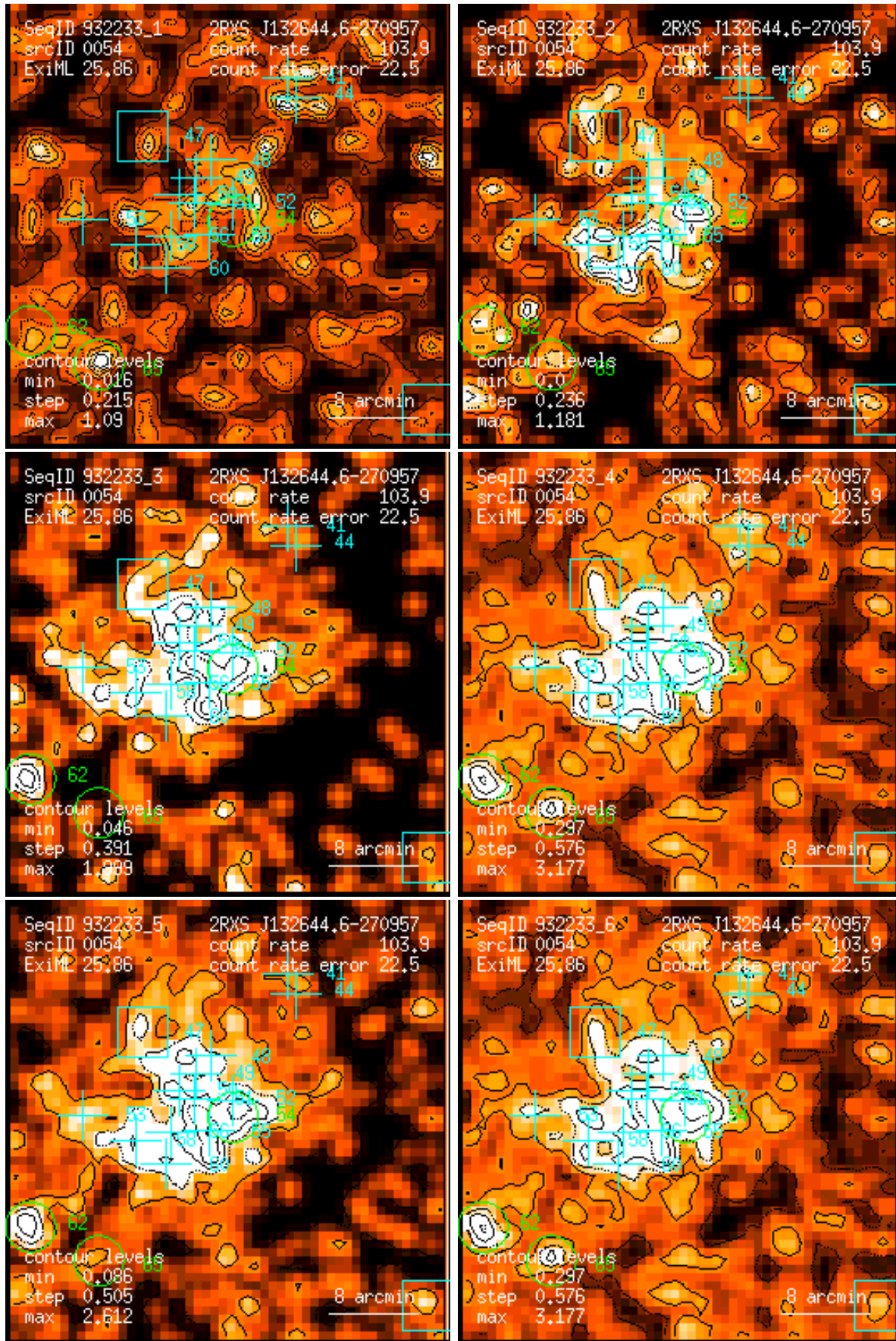
Figure 54: RASS 932233: detection 0054: band rate images, Gaussian filter: (1) PSPC channels 11 – 41, (2) 52 – 90, (3) 91 – 201, (4) 11 – 235, (5) 52 – 201, (6) 11 – 201. Broad band rates in counts/ks. Band rate contour levels in counts/ks/arcmin 2 .
