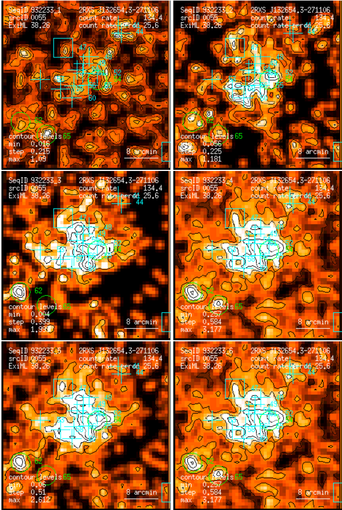
Figure 55: RASS 932233: detection 0055: band rate images, Gaussian filter: (1) PSPC channels 11 – 41, (2) 52 – 90, (3) 91 – 201, (4) 11 – 235, (5) 52 – 201, (6) 11 – 201. Broad band rates in counts/ks. Band rate contour levels in counts/ks/arcmin 2 .
