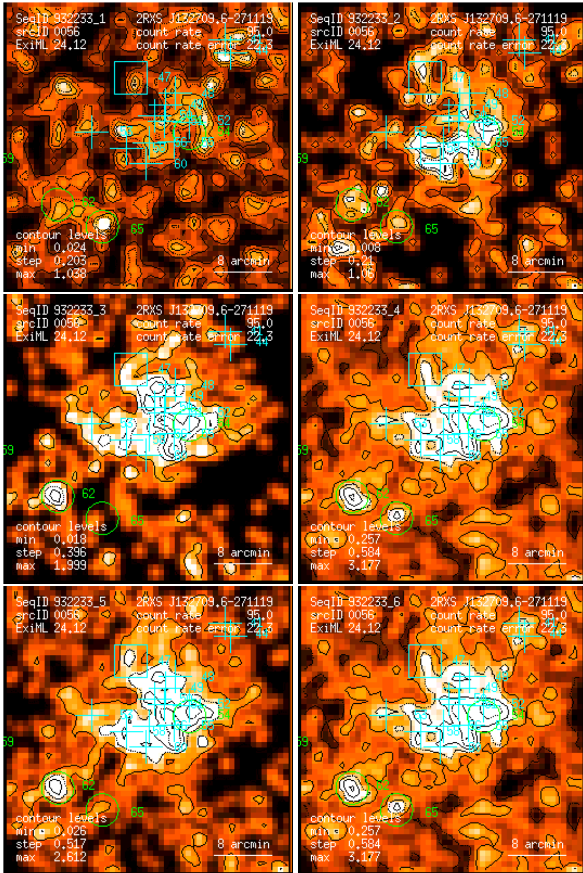
Figure 56: RASS 932233: detection 0056: band rate images, Gaussian filter: (1) PSPC channels 11 – 41, (2) 52 – 90, (3) 91 – 201, (4) 11 – 235, (5) 52 – 201, (6) 11 – 201. Broad band rates in counts/ks. Band rate contour levels in counts/ks/arcmin 2 .
