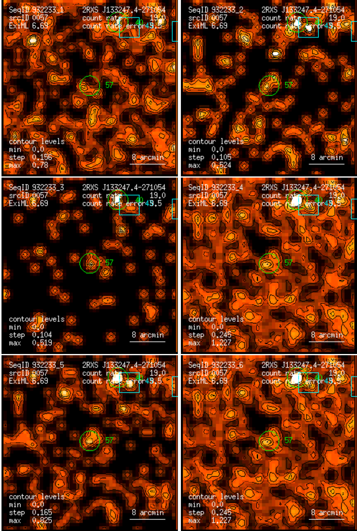
Figure 57: RASS 932233: detection 0057: band rate images, Gaussian filter: (1) PSPC channels 11 – 41, (2) 52 – 90, (3) 91 – 201, (4) 11 – 235, (5) 52 – 201, (6) 11 – 201. Broad band rates in counts/ks. Band rate contour levels in counts/ks/arcmin 2 .
