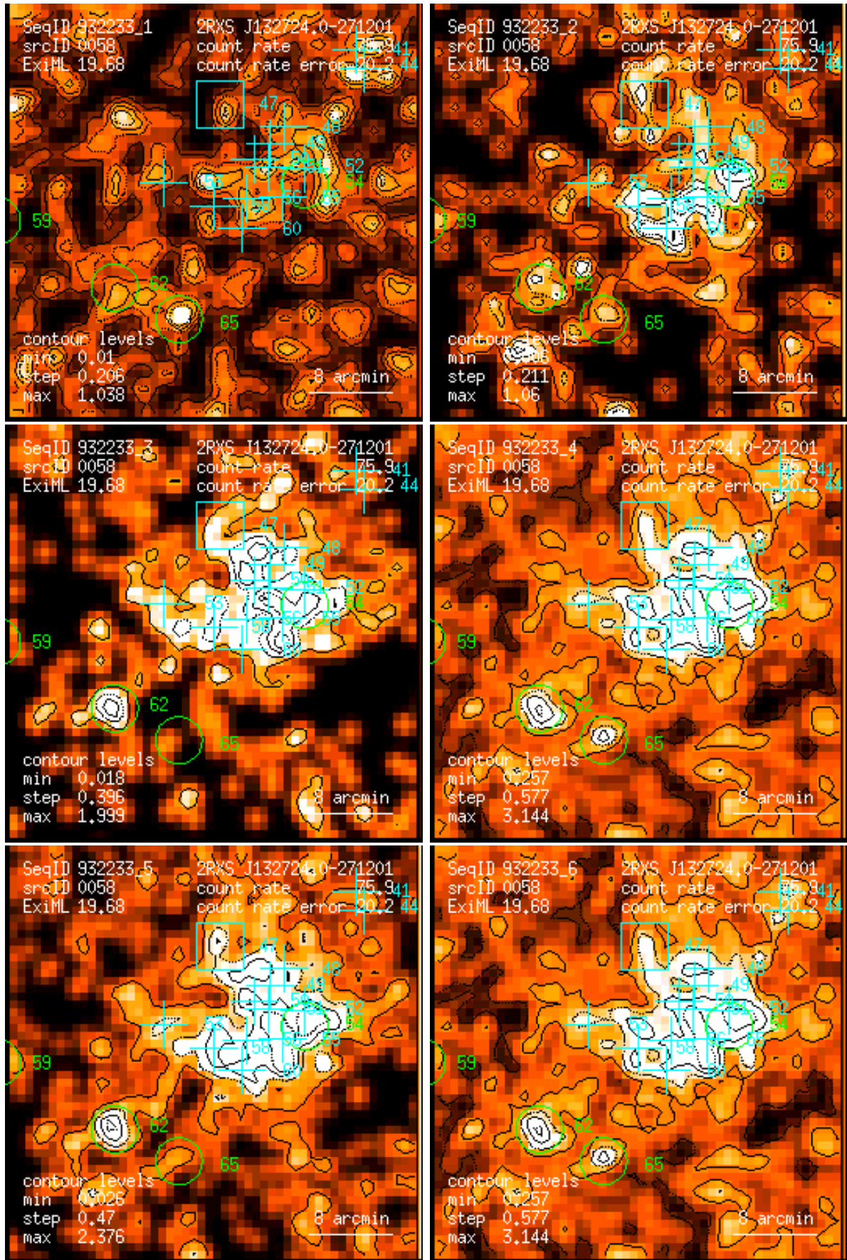
Figure 58: RASS 932233: detection 0058: band rate images, Gaussian filter: (1) PSPC channels 11 – 41, (2) 52 – 90, (3) 91 – 201, (4) 11 – 235, (5) 52 – 201, (6) 11 – 201. Broad band rates in counts/ks. Band rate contour levels in counts/ks/arcmin 2 .
