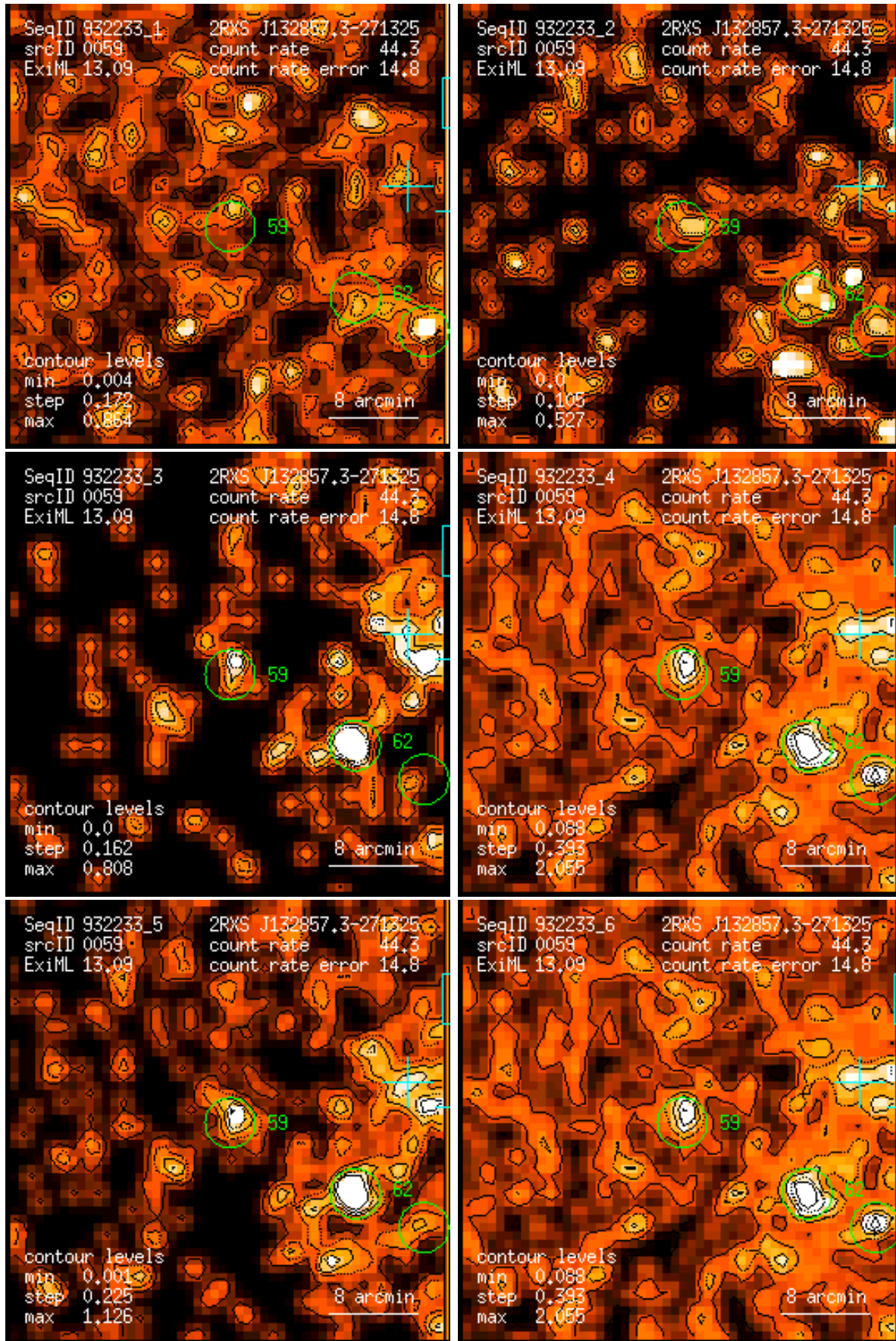
Figure 59: RASS 932233: detection 0059: band rate images, Gaussian filter: (1) PSPC channels 11 – 41, (2) 52 – 90, (3) 91 – 201, (4) 11 – 235, (5) 52 – 201, (6) 11 – 201. Broad band rates in counts/ks. Band rate contour levels in counts/ks/arcmin 2 .
