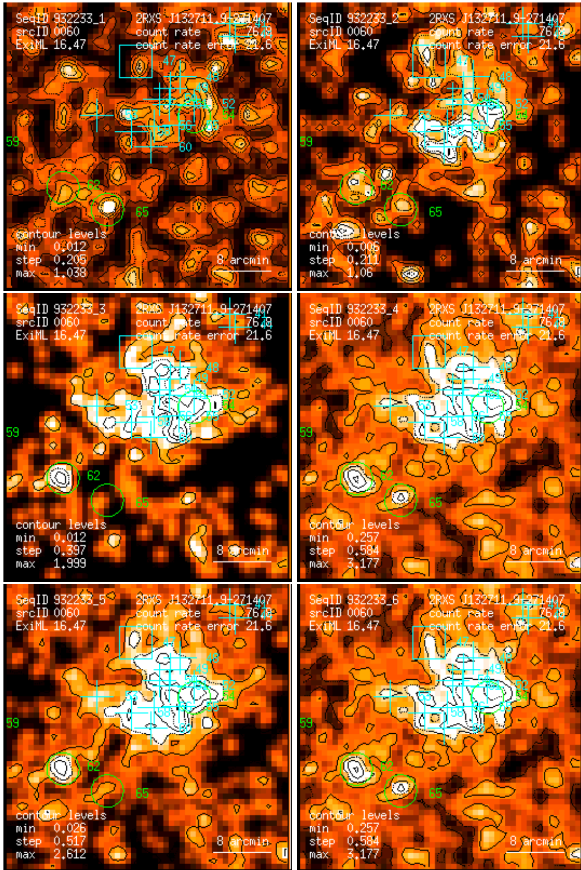
Figure 60: RASS 932233: detection 0060: band rate images, Gaussian filter: (1) PSPC channels 11 – 41, (2) 52 – 90, (3) 91 – 201, (4) 11 – 235, (5) 52 – 201, (6) 11 – 201. Broad band rates in counts/ks. Band rate contour levels in counts/ks/arcmin 2 .
