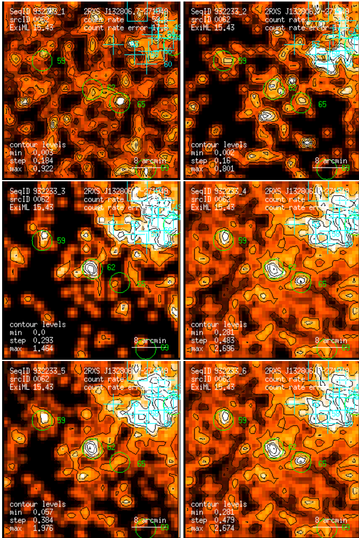
Figure 62: RASS 932233: detection 0062: band rate images, Gaussian filter: (1) PSPC channels 11 – 41, (2) 52 – 90, (3) 91 – 201, (4) 11 – 235, (5) 52 – 201, (6) 11 – 201. Broad band rates in counts/ks. Band rate contour levels in counts/ks/arcmin 2 .
