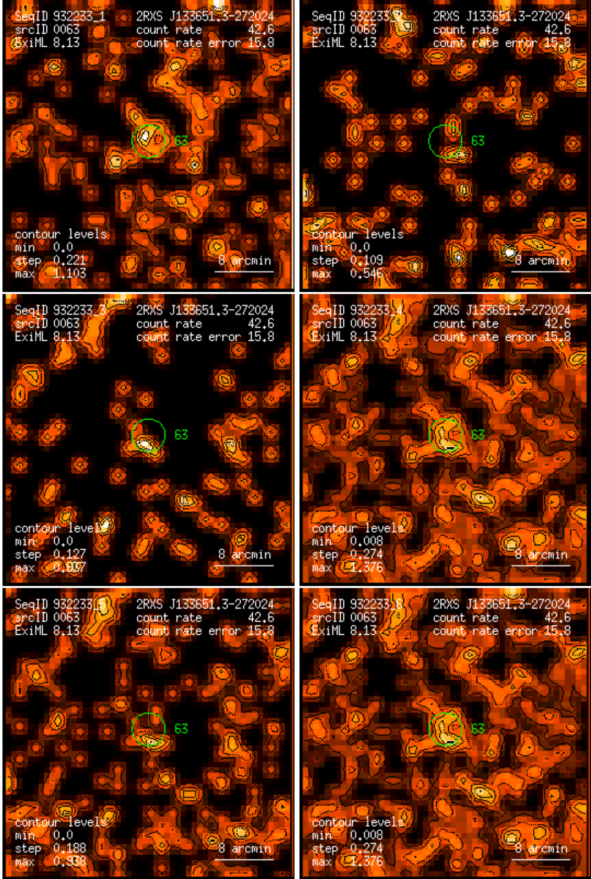
Figure 63: RASS 932233: detection 0063: band rate images, Gaussian filter: (1) PSPC channels 11 – 41, (2) 52 – 90, (3) 91 – 201, (4) 11 – 235, (5) 52 – 201, (6) 11 – 201. Broad band rates in counts/ks. Band rate contour levels in counts/ks/arcmin 2 .
