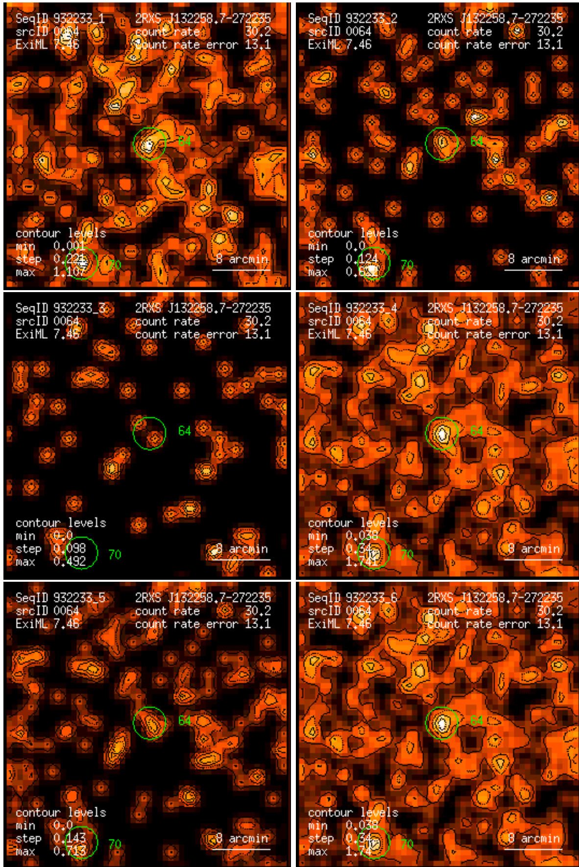
Figure 64: RASS 932233: detection 0064: band rate images, Gaussian filter: (1) PSPC channels 11 – 41, (2) 52 – 90, (3) 91 – 201, (4) 11 – 235, (5) 52 – 201, (6) 11 – 201. Broad band rates in counts/ks. Band rate contour levels in counts/ks/arcmin 2 .
