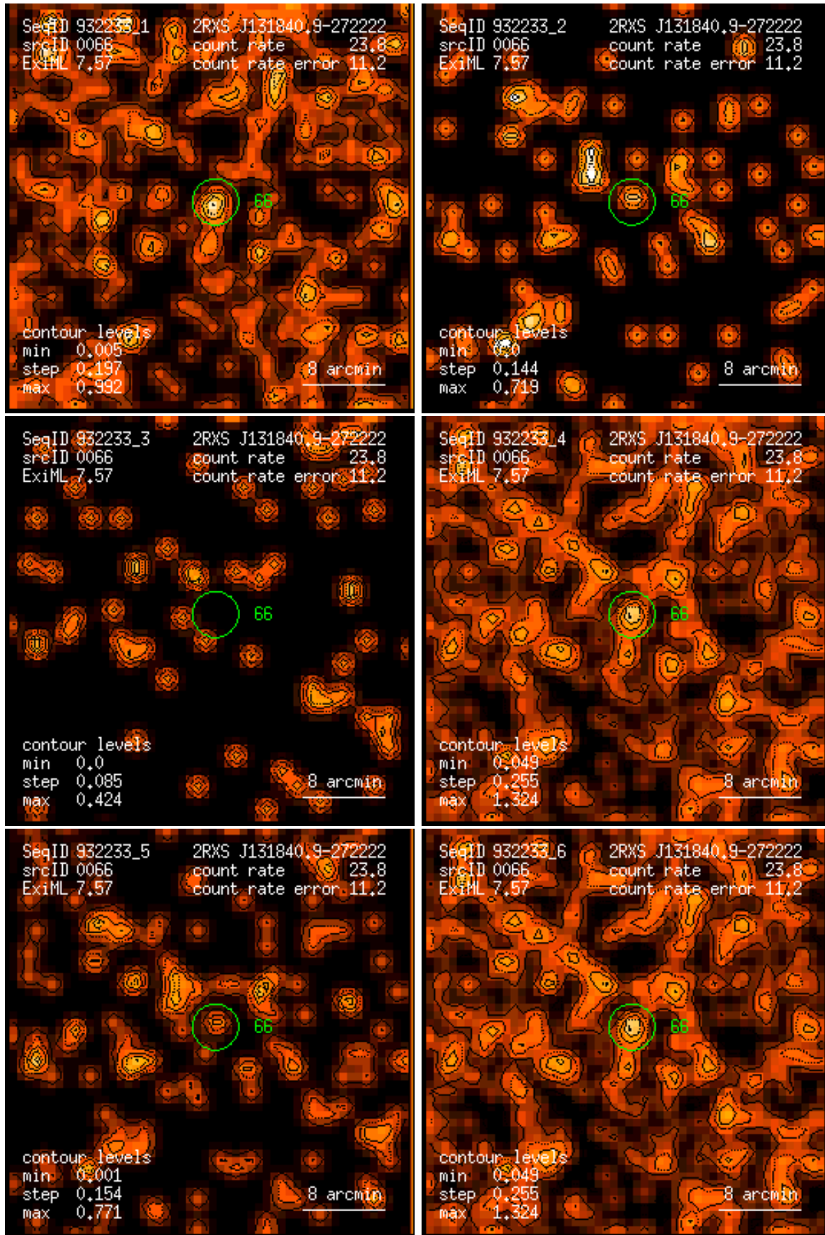
Figure 66: RASS 932233: detection 0066: band rate images, Gaussian filter: (1) PSPC channels 11 – 41, (2) 52 – 90, (3) 91 – 201, (4) 11 – 235, (5) 52 – 201, (6) 11 – 201. Broad band rates in counts/ks. Band rate contour levels in counts/ks/arcmin 2 .
