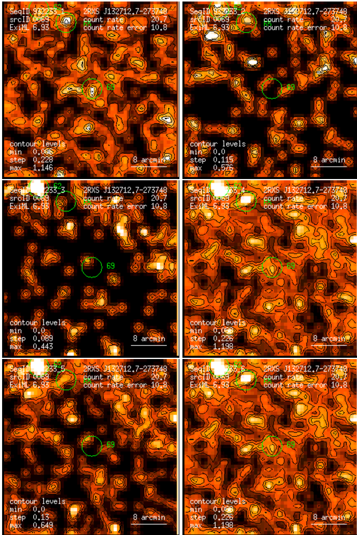
Figure 69: RASS 932233: detection 0069: band rate images, Gaussian filter: (1) PSPC channels 11 – 41, (2) 52 – 90, (3) 91 – 201, (4) 11 – 235, (5) 52 – 201, (6) 11 – 201. Broad band rates in counts/ks. Band rate contour levels in counts/ks/arcmin 2 .
