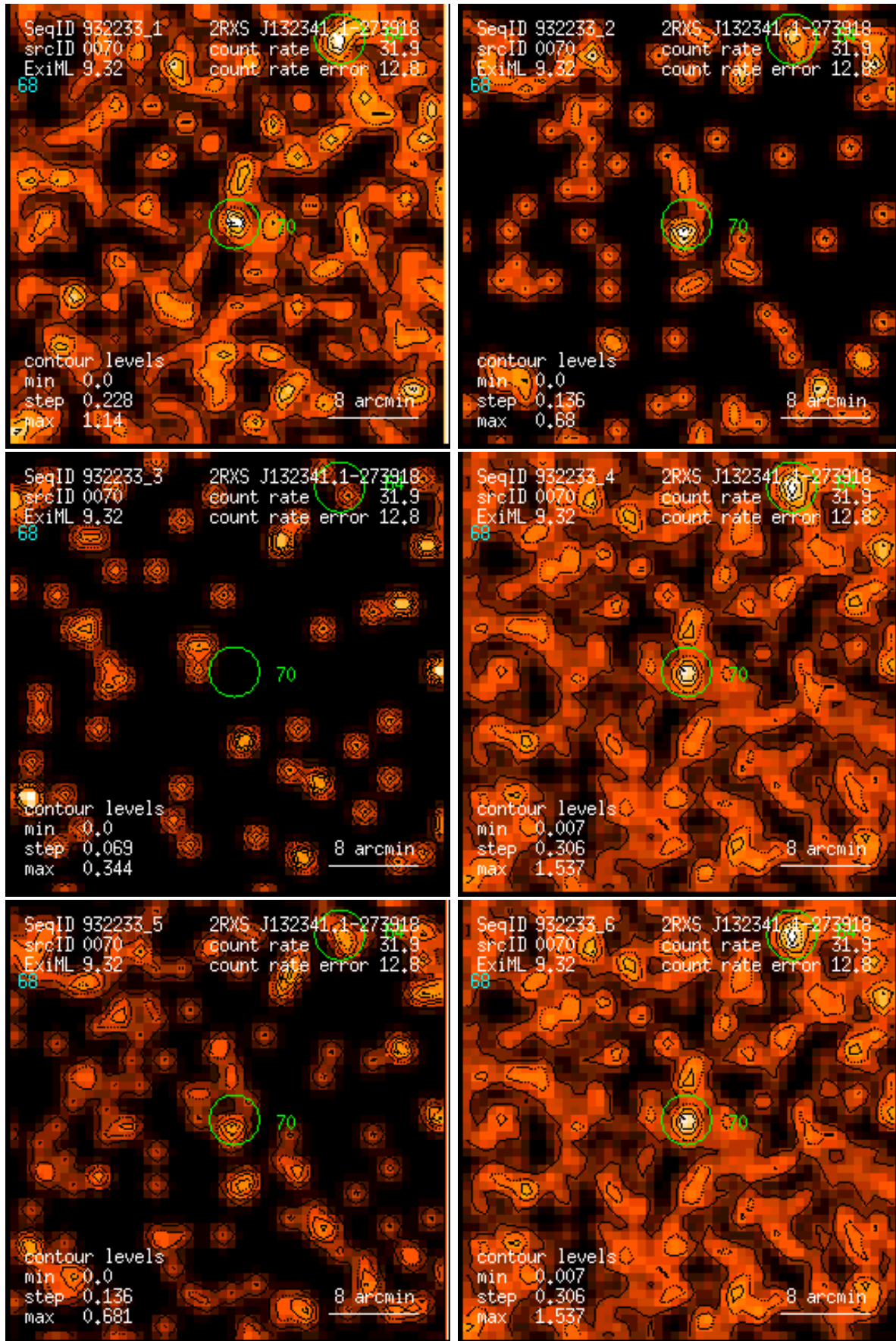
Figure 70: RASS 932233: detection 0070: band rate images, Gaussian filter: (1) PSPC channels 11 – 41, (2) 52 – 90, (3) 91 – 201, (4) 11 – 235, (5) 52 – 201, (6) 11 – 201. Broad band rates in counts/ks. Band rate contour levels in counts/ks/arcmin 2 .
