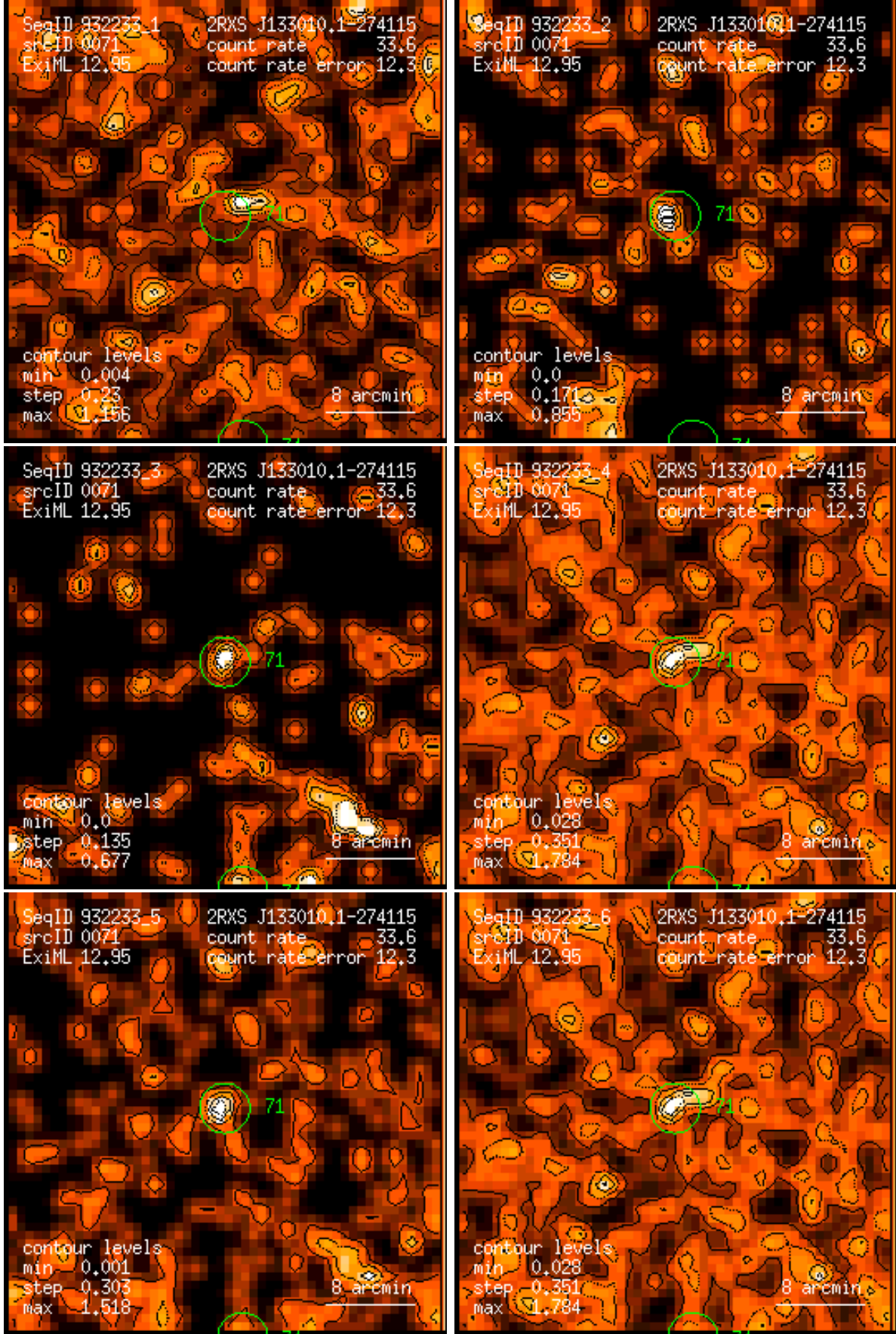
Figure 71: RASS 932233: detection 0071: band rate images, Gaussian filter: (1) PSPC channels 11 – 41, (2) 52 – 90, (3) 91 – 201, (4) 11 – 235, (5) 52 – 201, (6) 11 – 201. Broad band rates in counts/ks. Band rate contour levels in counts/ks/arcmin 2 .
