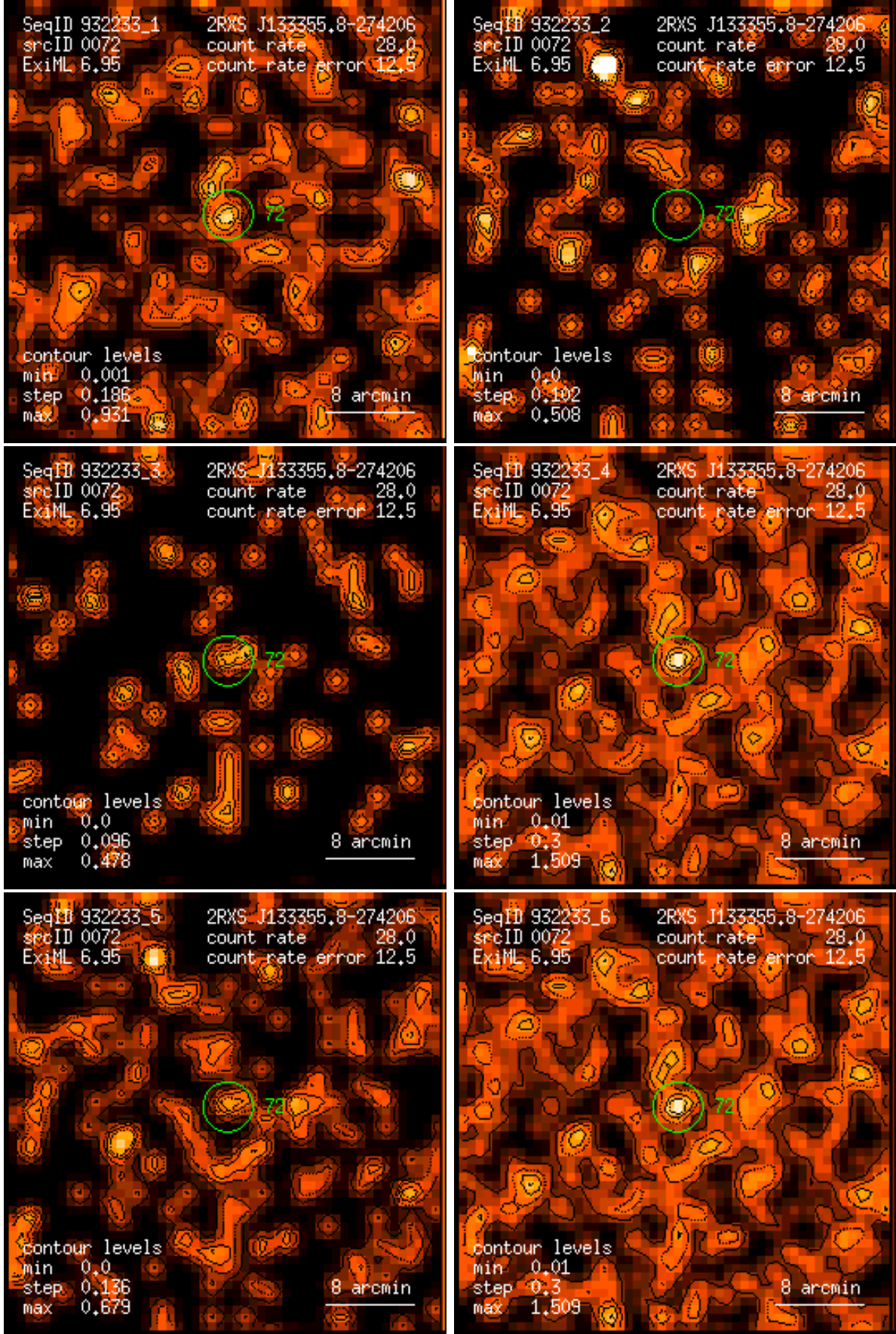
Figure 72: RASS 932233: detection 0072: band rate images, Gaussian filter: (1) PSPC channels 11 – 41, (2) 52 – 90, (3) 91 – 201, (4) 11 – 235, (5) 52 – 201, (6) 11 – 201. Broad band rates in counts/ks. Band rate contour levels in counts/ks/arcmin 2 .
