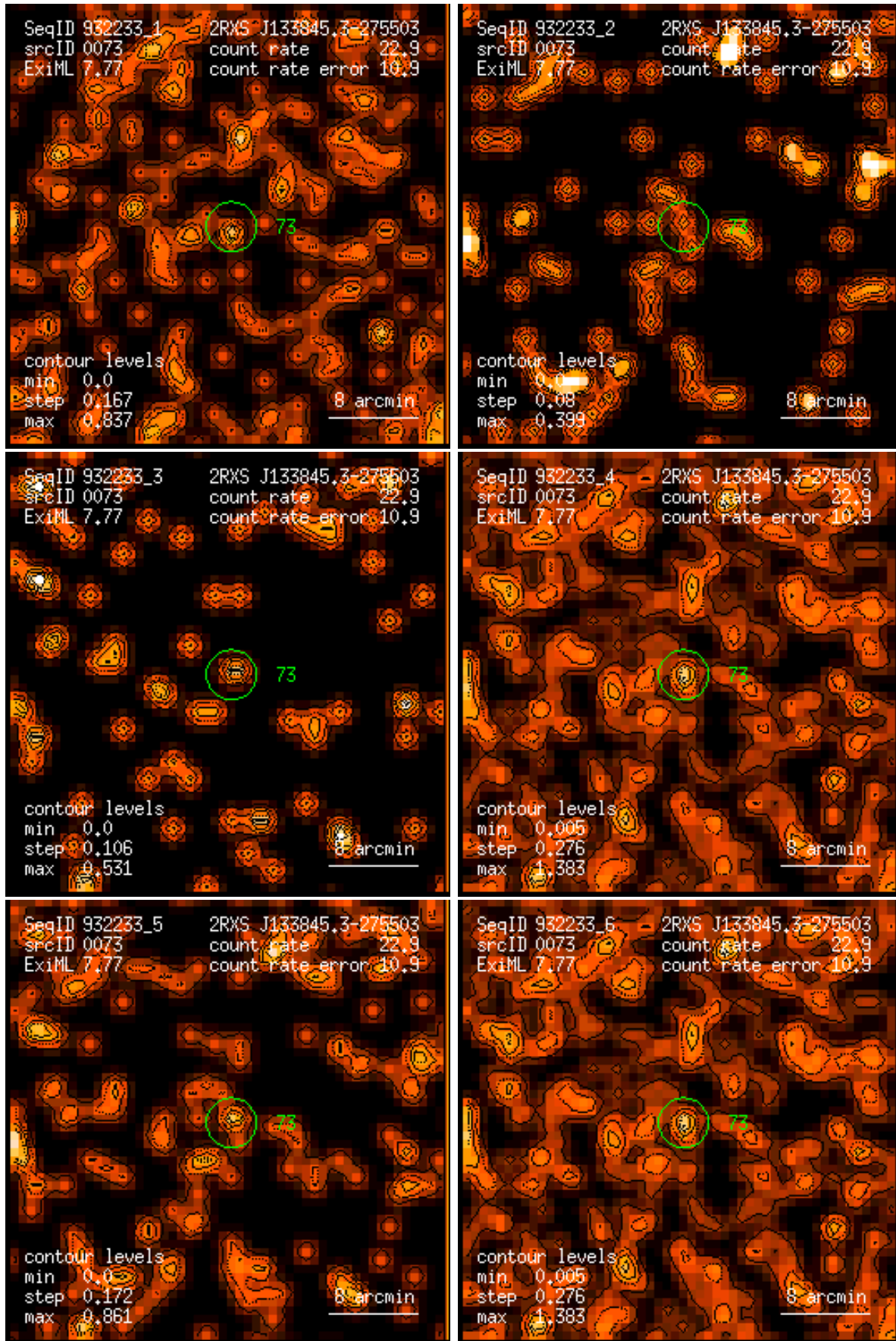
Figure 73: RASS 932233: detection 0073: band rate images, Gaussian filter: (1) PSPC channels 11 – 41, (2) 52 – 90, (3) 91 – 201, (4) 11 – 235, (5) 52 – 201, (6) 11 – 201. Broad band rates in counts/ks. Band rate contour levels in counts/ks/arcmin 2 .
