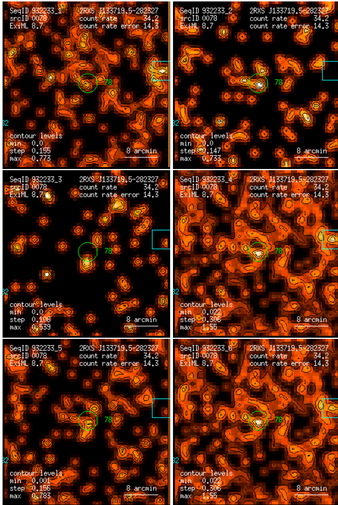
Figure 78: RASS 932233: detection 0078: band rate images, Gaussian filter: (1) PSPC channels 11 – 41, (2) 52 – 90, (3) 91 – 201, (4) 11 – 235, (5) 52 – 201, (6) 11 – 201. Broad band rates in counts/ks. Band rate contour levels in counts/ks/arcmin 2 .
