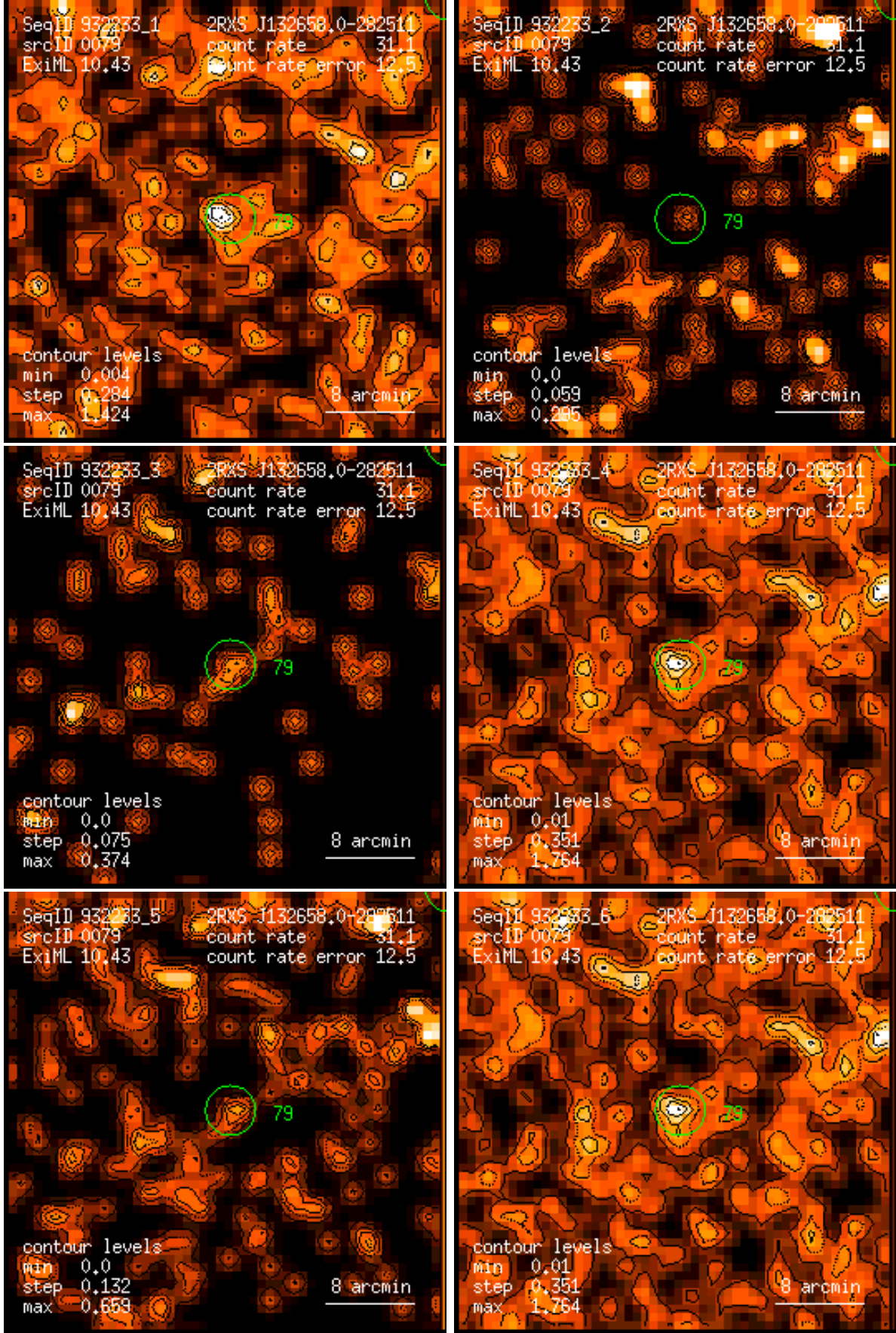
Figure 79: RASS 932233: detection 0079: band rate images, Gaussian filter: (1) PSPC channels 11 – 41, (2) 52 – 90, (3) 91 – 201, (4) 11 – 235, (5) 52 – 201, (6) 11 – 201. Broad band rates in counts/ks. Band rate contour levels in counts/ks/arcmin 2 .
