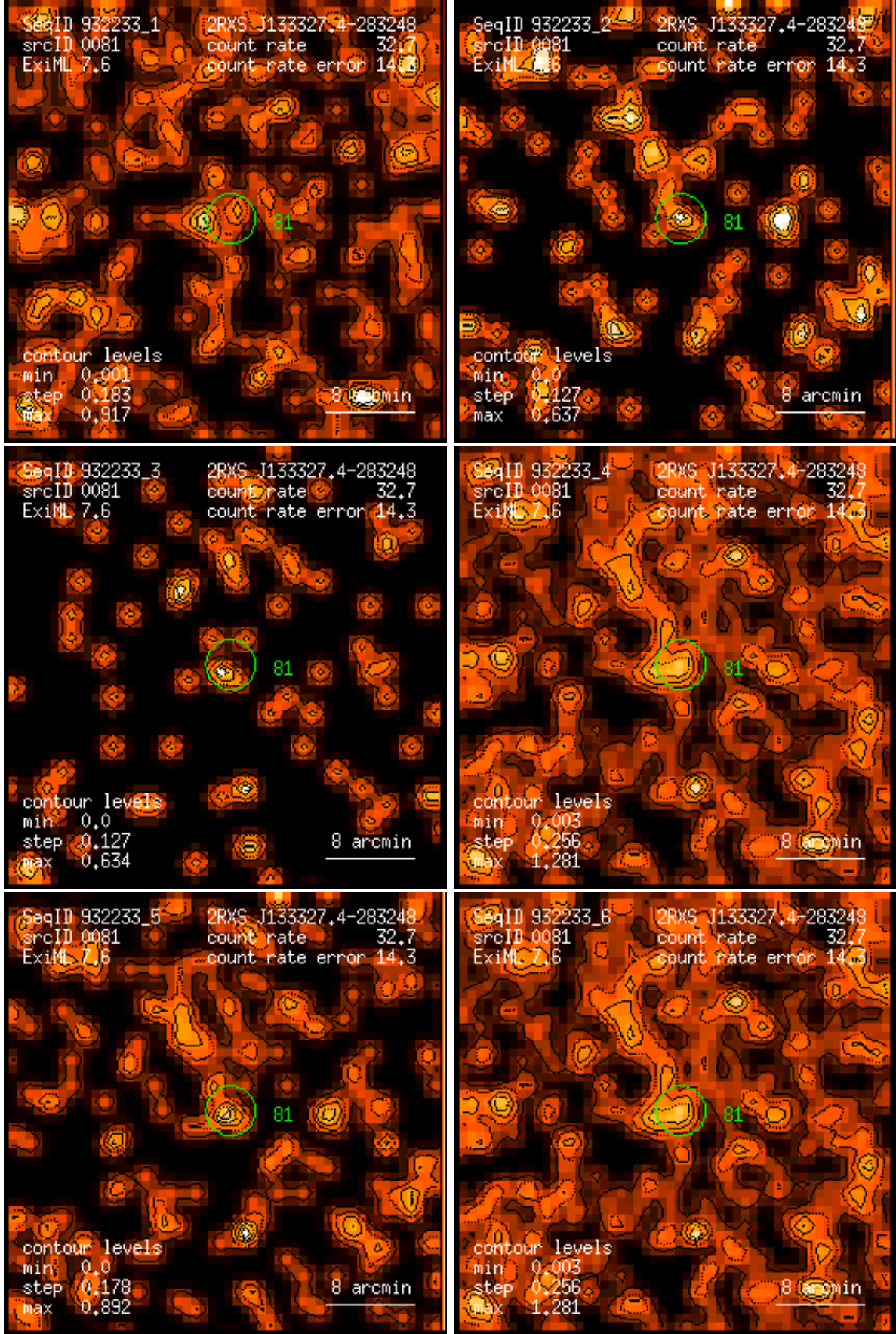
Figure 81: RASS 932233: detection 0081: band rate images, Gaussian filter: (1) PSPC channels 11 – 41, (2) 52 – 90, (3) 91 – 201, (4) 11 – 235, (5) 52 – 201, (6) 11 – 201. Broad band rates in counts/ks. Band rate contour levels in counts/ks/arcmin 2 .
