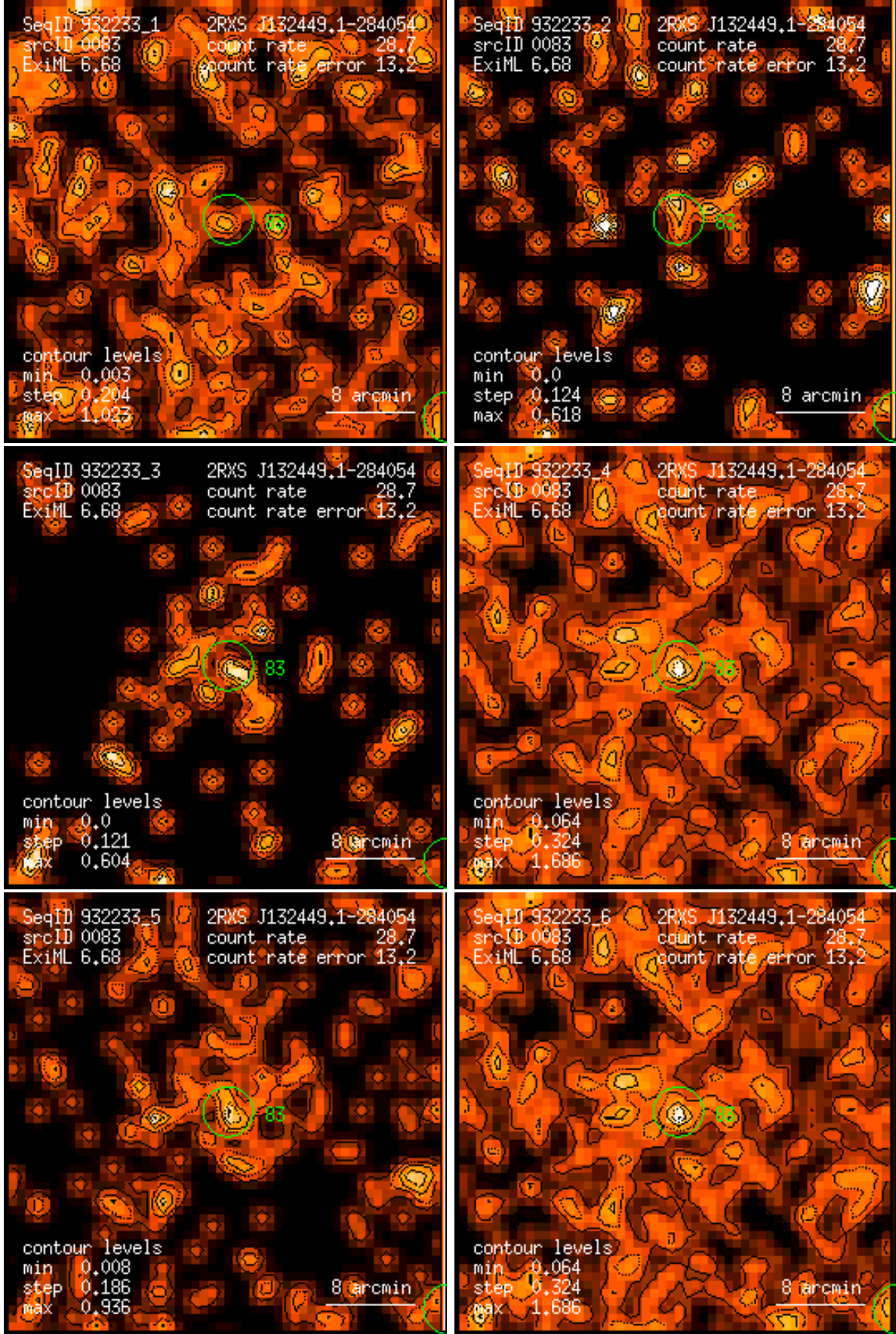
Figure 83: RASS 932233: detection 0083: band rate images, Gaussian filter: (1) PSPC channels 11 – 41, (2) 52 – 90, (3) 91 – 201, (4) 11 – 235, (5) 52 – 201, (6) 11 – 201. Broad band rates in counts/ks. Band rate contour levels in counts/ks/arcmin 2 .
