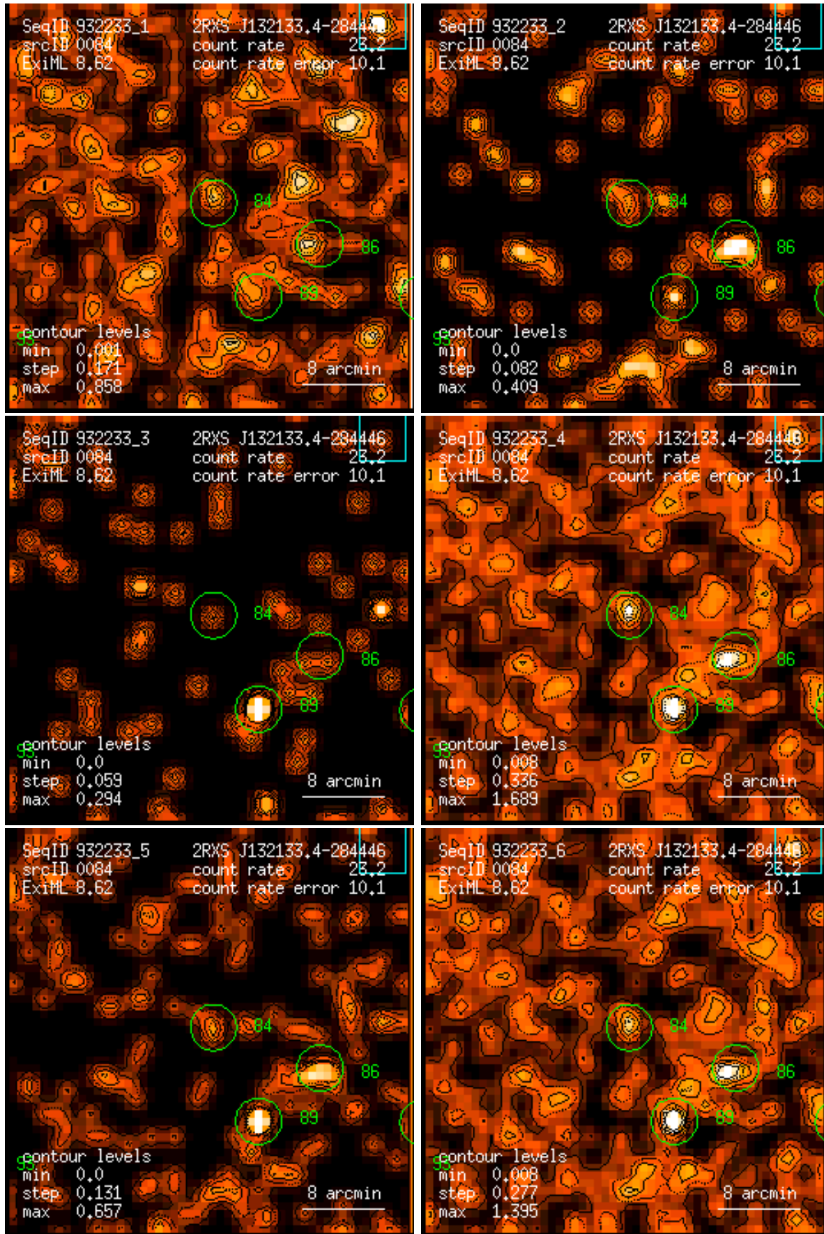
Figure 84: RASS 932233: detection 0084: band rate images, Gaussian filter: (1) PSPC channels 11 – 41, (2) 52 – 90, (3) 91 – 201, (4) 11 – 235, (5) 52 – 201, (6) 11 – 201. Broad band rates in counts/ks. Band rate contour levels in counts/ks/arcmin 2 .
