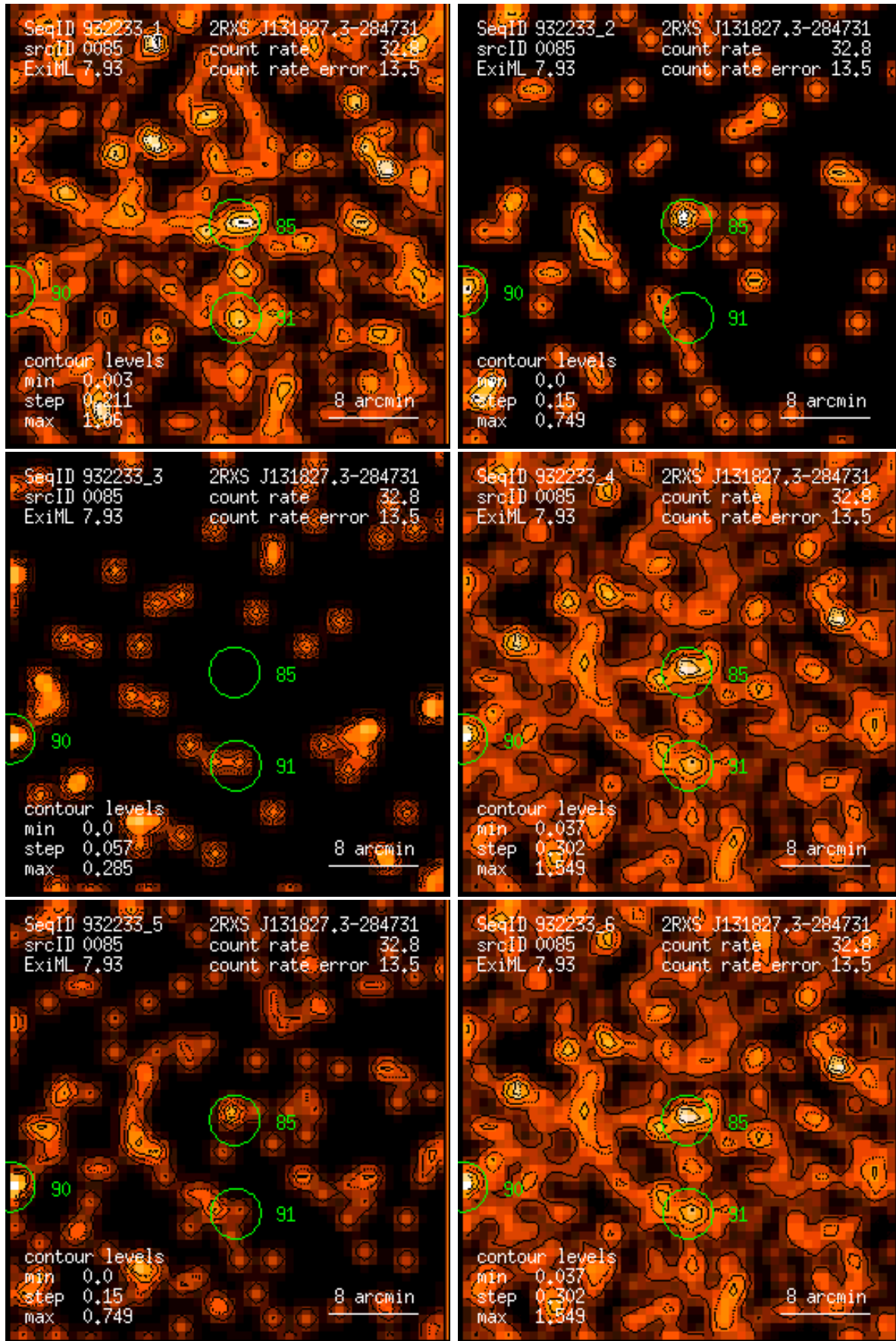
Figure 85: RASS 932233: detection 0085: band rate images, Gaussian filter: (1) PSPC channels 11 – 41, (2) 52 – 90, (3) 91 – 201, (4) 11 – 235, (5) 52 – 201, (6) 11 – 201. Broad band rates in counts/ks. Band rate contour levels in counts/ks/arcmin 2 .
