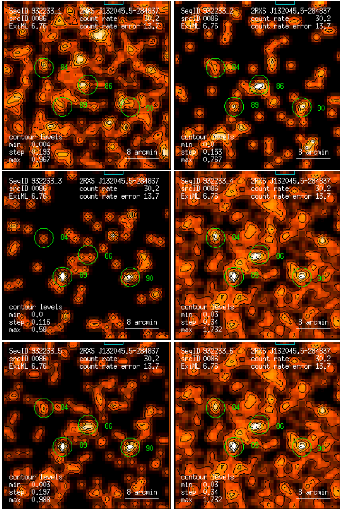
Figure 86: RASS 932233: detection 0086: band rate images, Gaussian filter: (1) PSPC channels 11 – 41, (2) 52 – 90, (3) 91 – 201, (4) 11 – 235, (5) 52 – 201, (6) 11 – 201. Broad band rates in counts/ks. Band rate contour levels in counts/ks/arcmin 2 .
