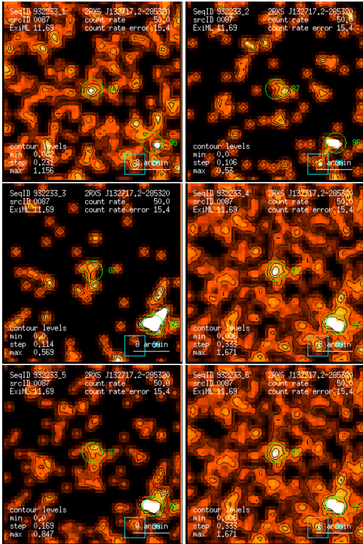
Figure 87: RASS 932233: detection 0087: band rate images, Gaussian filter: (1) PSPC channels 11 – 41, (2) 52 – 90, (3) 91 – 201, (4) 11 – 235, (5) 52 – 201, (6) 11 – 201. Broad band rates in counts/ks. Band rate contour levels in counts/ks/arcmin 2 .
