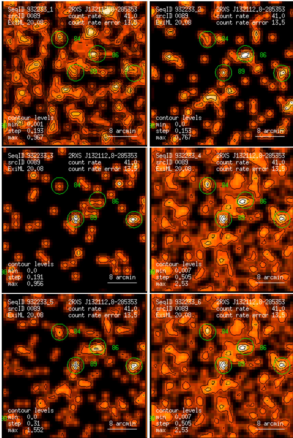
Figure 89: RASS 932233: detection 0089: band rate images, Gaussian filter: (1) PSPC channels 11 – 41, (2) 52 – 90, (3) 91 – 201, (4) 11 – 235, (5) 52 – 201, (6) 11 – 201. Broad band rates in counts/ks. Band rate contour levels in counts/ks/arcmin 2 .
