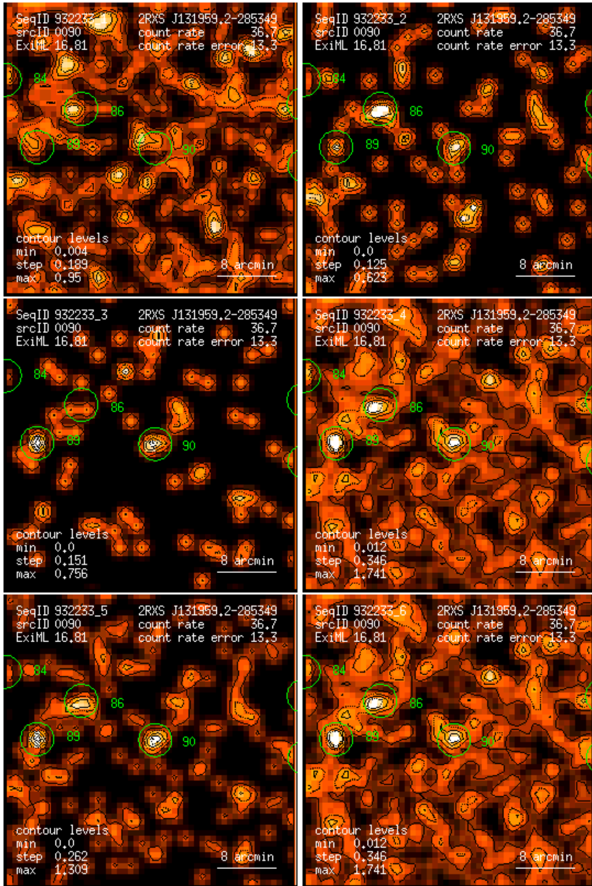
Figure 90: RASS 932233: detection 0090: band rate images, Gaussian filter: (1) PSPC channels 11 – 41, (2) 52 – 90, (3) 91 – 201, (4) 11 – 235, (5) 52 – 201, (6) 11 – 201. Broad band rates in counts/ks. Band rate contour levels in counts/ks/arcmin 2 .
