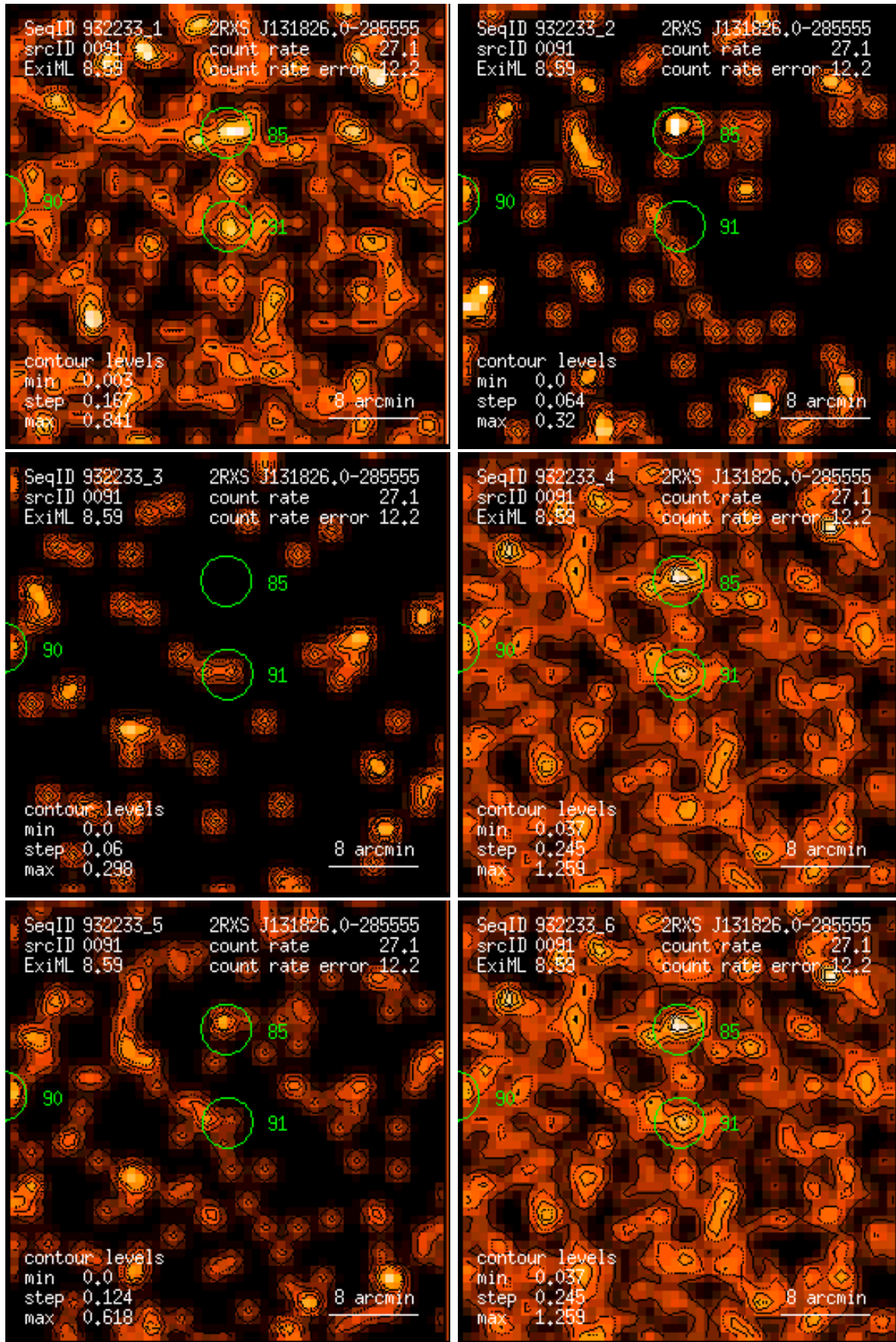
Figure 91: RASS 932233: detection 0091: band rate images, Gaussian filter: (1) PSPC channels 11 – 41, (2) 52 – 90, (3) 91 – 201, (4) 11 – 235, (5) 52 – 201, (6) 11 – 201. Broad band rates in counts/ks. Band rate contour levels in counts/ks/arcmin 2 .
