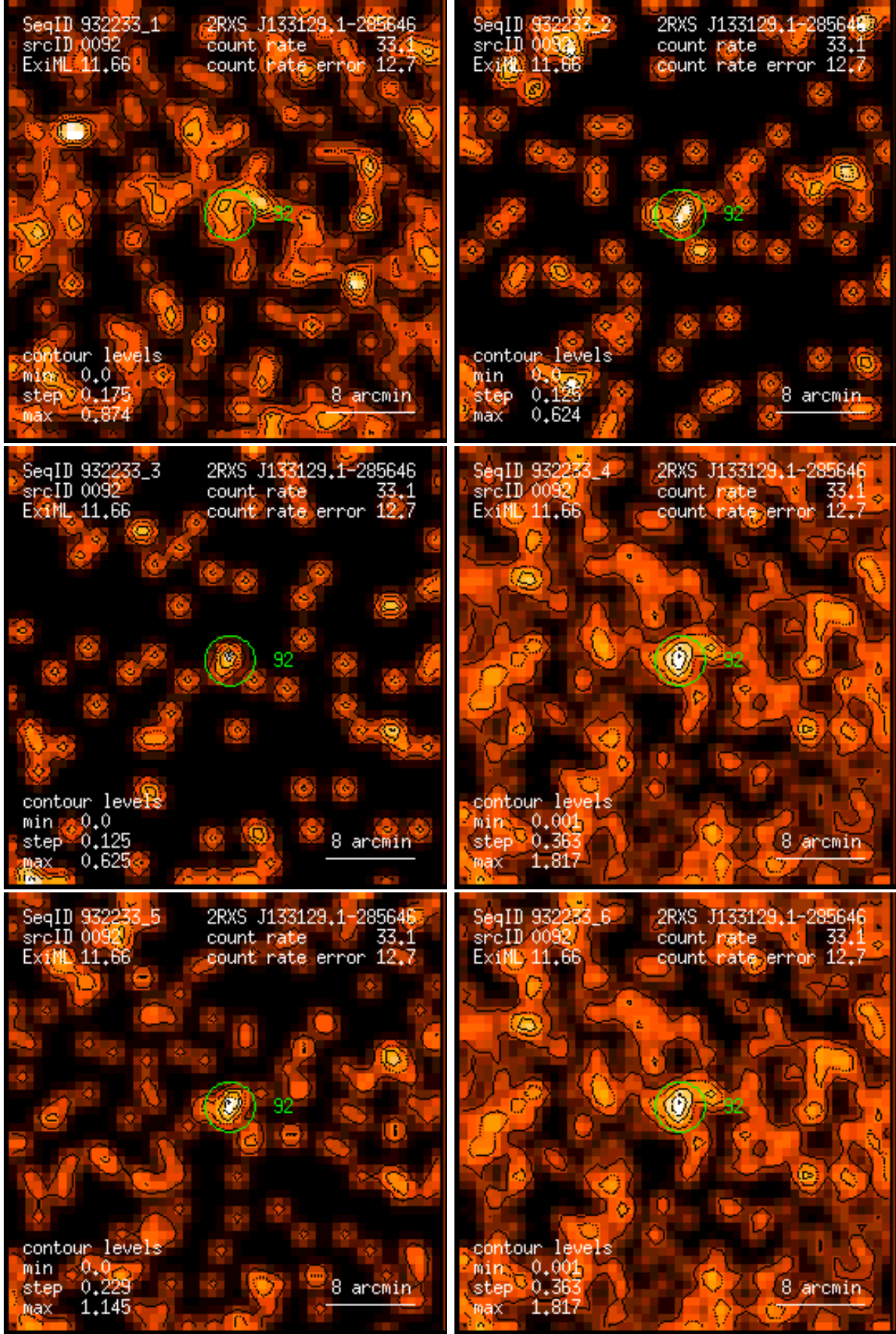
Figure 92: RASS 932233: detection 0092: band rate images, Gaussian filter: (1) PSPC channels 11 – 41, (2) 52 – 90, (3) 91 – 201, (4) 11 – 235, (5) 52 – 201, (6) 11 – 201. Broad band rates in counts/ks. Band rate contour levels in counts/ks/arcmin 2 .
