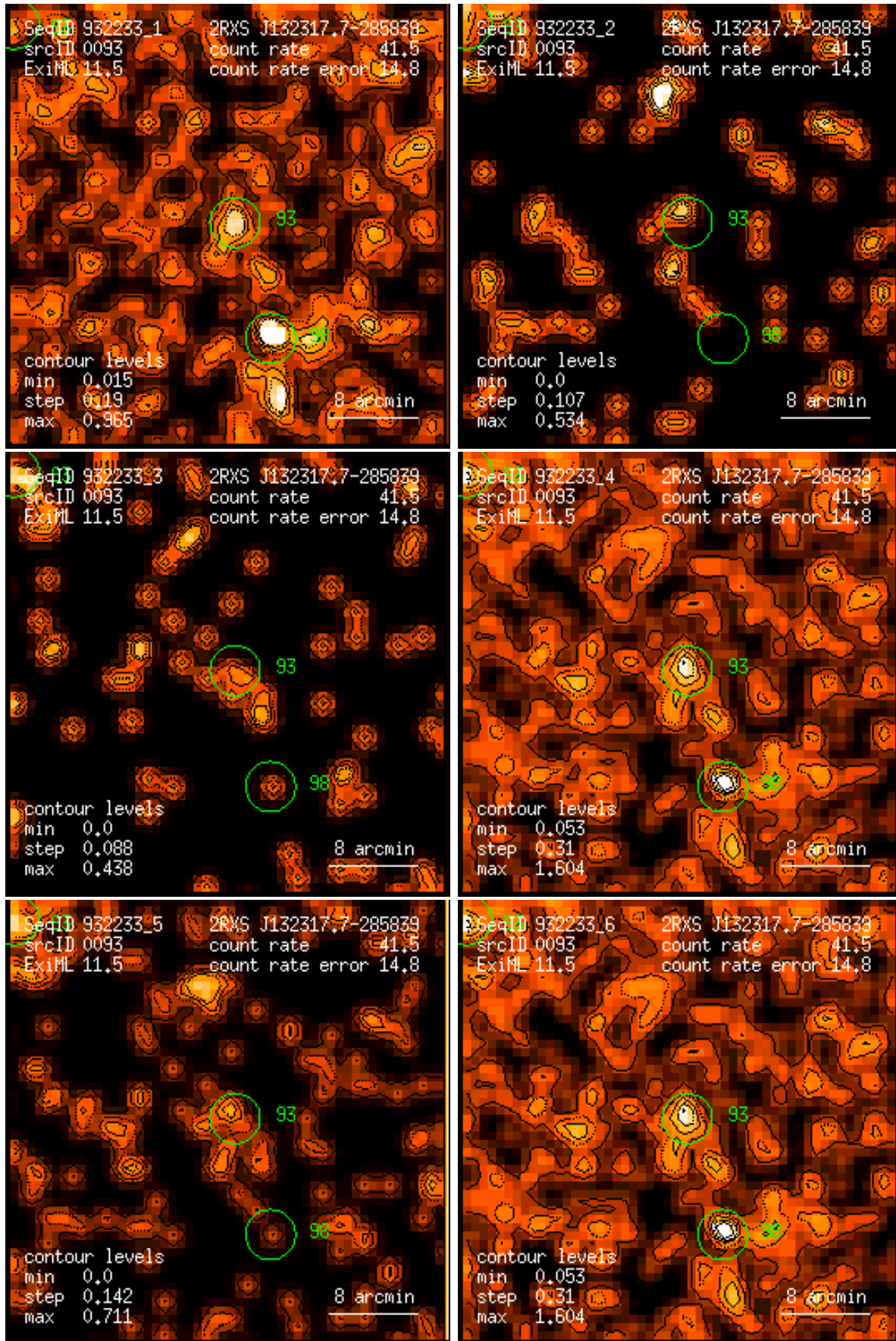
Figure 93: RASS 932233: detection 0093: band rate images, Gaussian filter: (1) PSPC channels 11 – 41, (2) 52 – 90, (3) 91 – 201, (4) 11 – 235, (5) 52 – 201, (6) 11 – 201. Broad band rates in counts/ks. Band rate contour levels in counts/ks/arcmin 2 .
