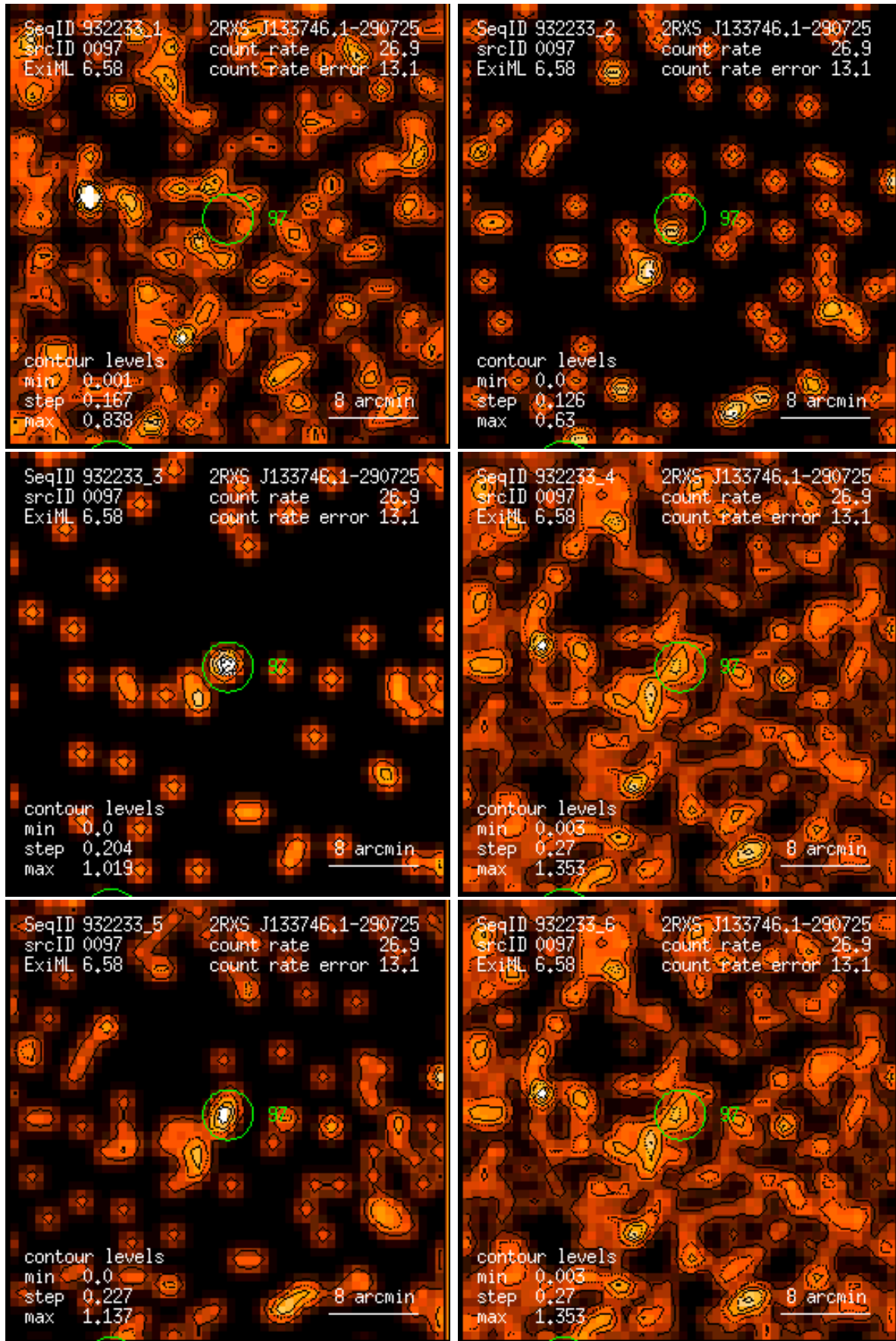
Figure 97: RASS 932233: detection 0097: band rate images, Gaussian filter: (1) PSPC channels 11 – 41, (2) 52 – 90, (3) 91 – 201, (4) 11 – 235, (5) 52 – 201, (6) 11 – 201. Broad band rates in counts/ks. Band rate contour levels in counts/ks/arcmin 2 .
