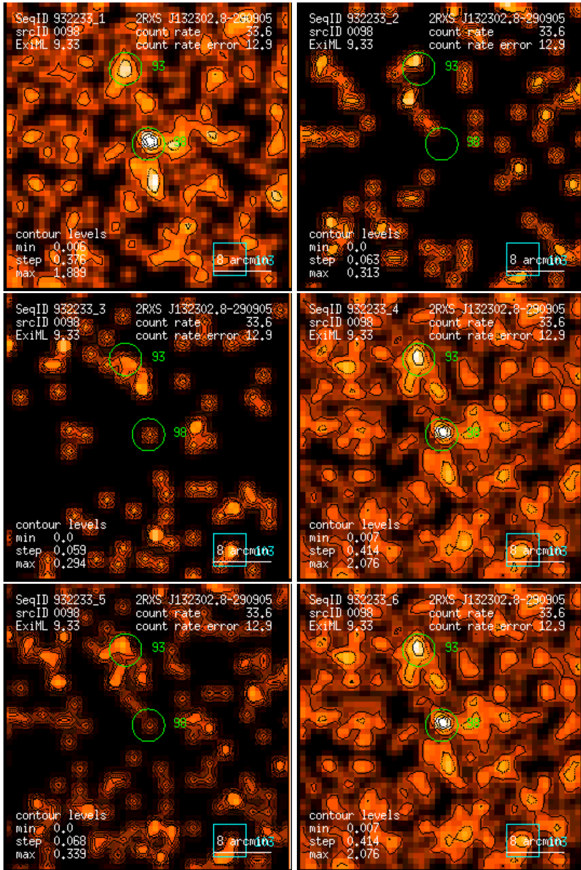
Figure 98: RASS 932233: detection 0098: band rate images, Gaussian filter: (1) PSPC channels 11 – 41, (2) 52 – 90, (3) 91 – 201, (4) 11 – 235, (5) 52 – 201, (6) 11 – 201. Broad band rates in counts/ks. Band rate contour levels in counts/ks/arcmin 2 .
