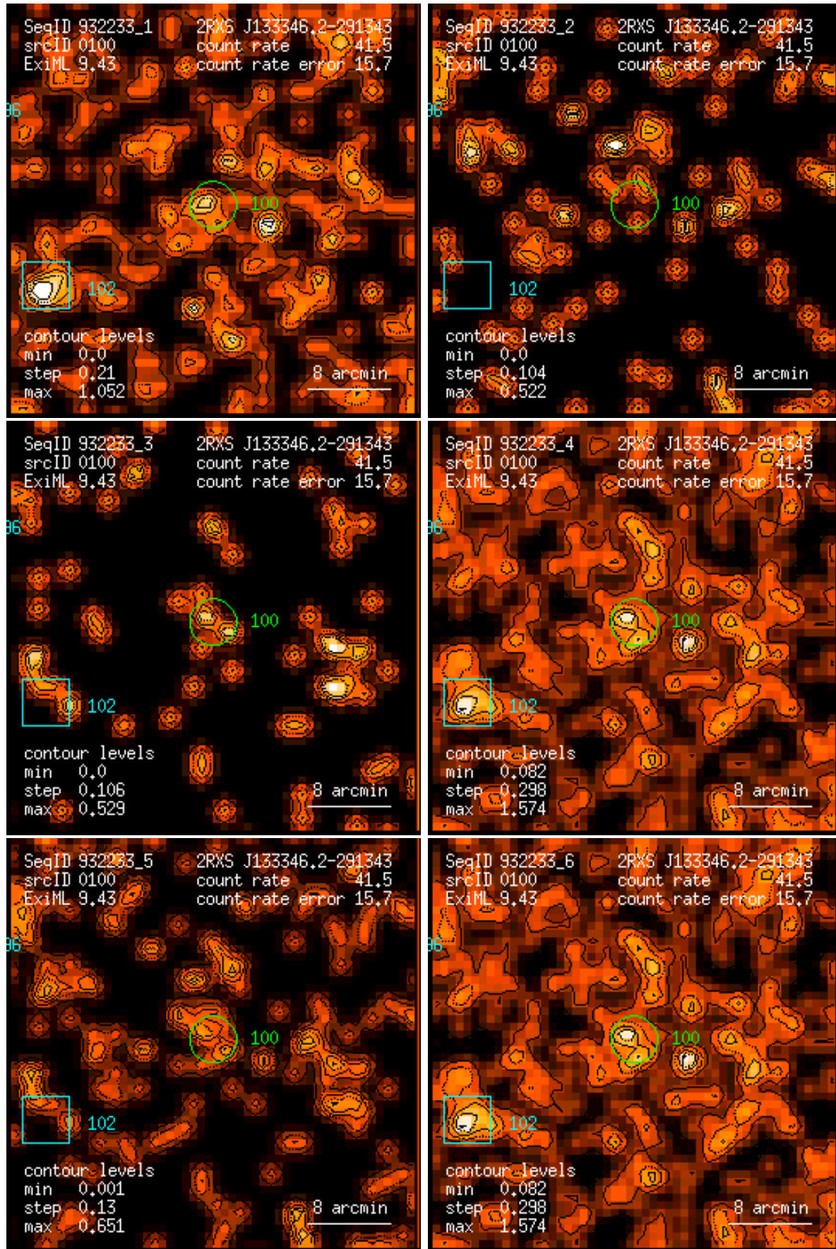
Figure 100: RASS 932233: detection 0100: band rate images, Gaussian filter: (1) PSPC channels 11 – 41, (2) 52 – 90, (3) 91 – 201, (4) 11 – 235, (5) 52 – 201, (6) 11 – 201. Broad band rates in counts/ks. Band rate contour levels in counts/ks/arcmin 2 .
