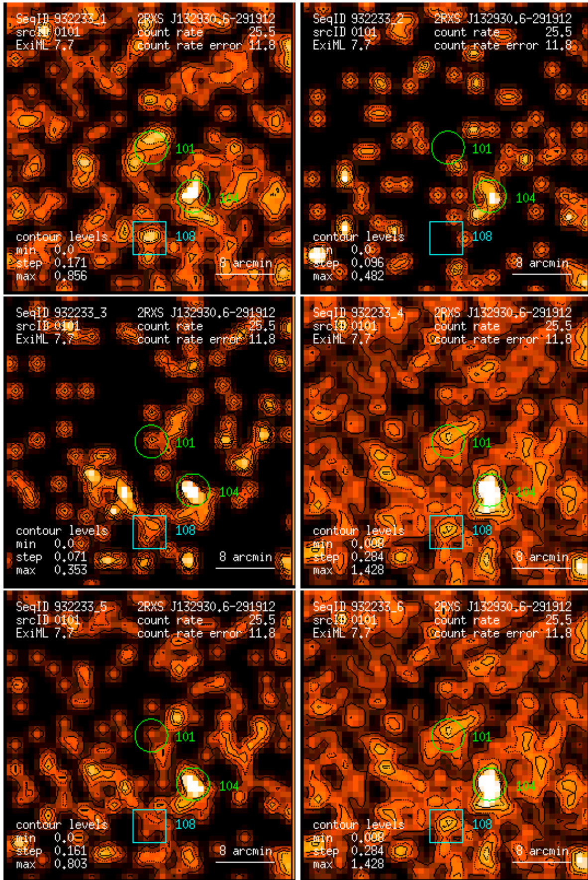
Figure 101: RASS 932233: detection 0101: band rate images, Gaussian filter: (1) PSPC channels 11 – 41, (2) 52 – 90, (3) 91 – 201, (4) 11 – 235, (5) 52 – 201, (6) 11 – 201. Broad band rates in counts/ks. Band rate contour levels in counts/ks/arcmin 2 .
