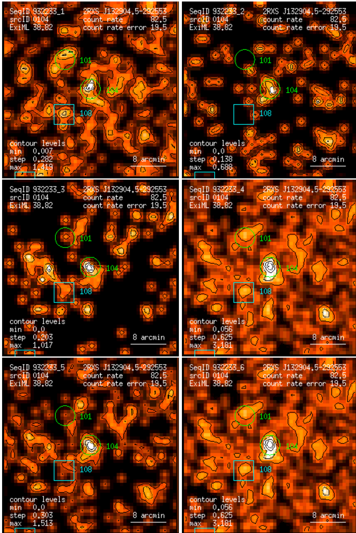
Figure 104: RASS 932233: detection 0104: band rate images, Gaussian filter: (1) PSPC channels 11 – 41, (2) 52 – 90, (3) 91 – 201, (4) 11 – 235, (5) 52 – 201, (6) 11 – 201. Broad band rates in counts/ks. Band rate contour levels in counts/ks/arcmin 2 .
