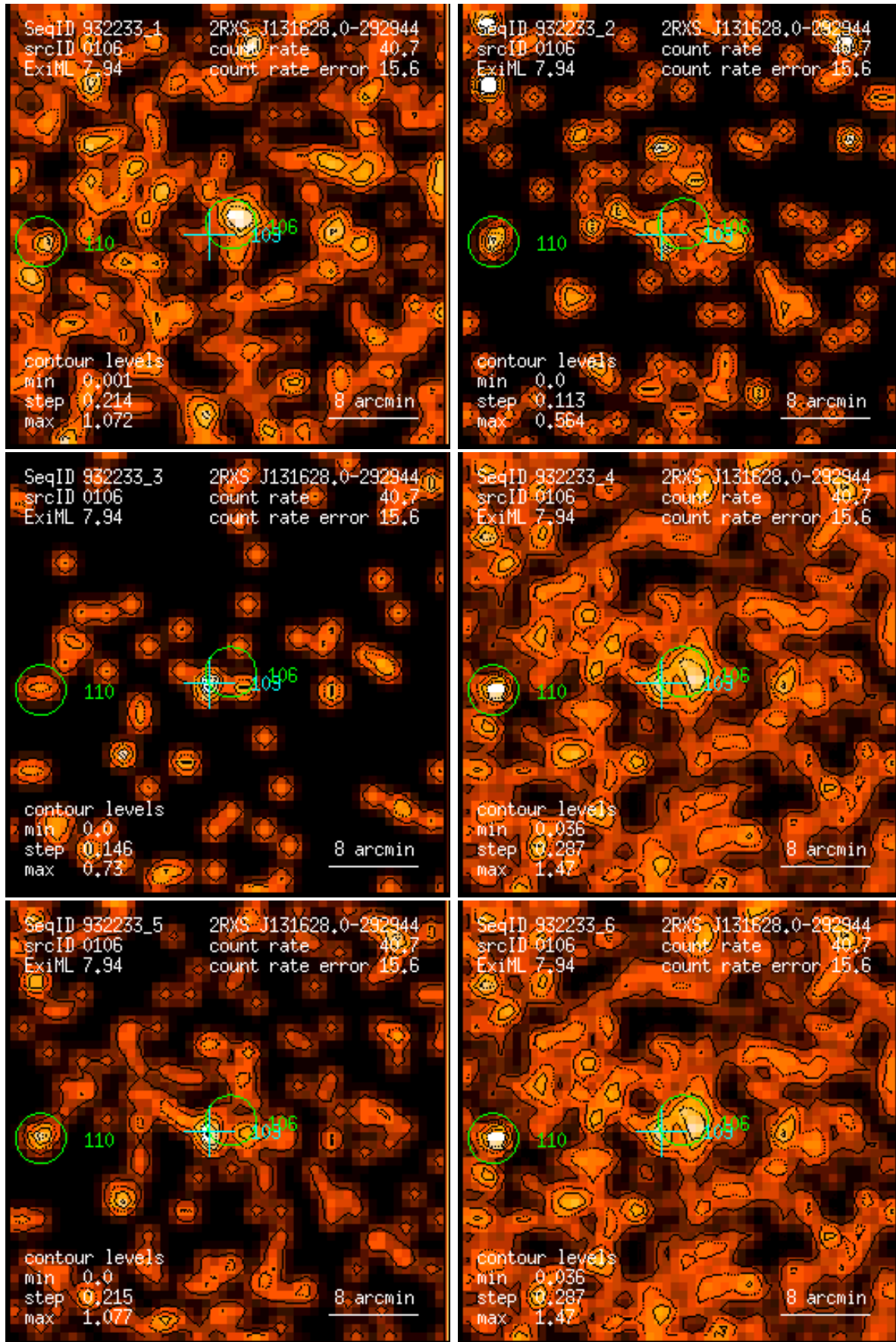
Figure 106: RASS 932233: detection 0106: band rate images, Gaussian filter: (1) PSPC channels 11 – 41, (2) 52 – 90, (3) 91 – 201, (4) 11 – 235, (5) 52 – 201, (6) 11 – 201. Broad band rates in counts/ks. Band rate contour levels in counts/ks/arcmin 2 .
